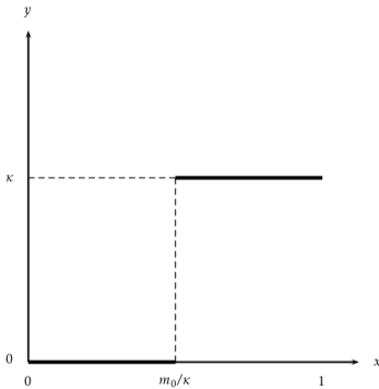
FIGURE 9. A solution of (II) in 1D, for large diffusivities \mu .
