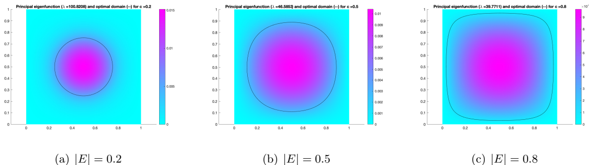
FIGURE 3. \Omega = (0, 1)^2 . Optimal domains in the Dirichlet case with \kappa = 0.5 and several volume constraints on E . Colors correspond to the intensity levels of the eigenfunction and the domain E encloses the zone corresponding to the warmest colors. Note that we know by Theorem 2 that the boundaries of the patterns observed in (a), (b) and (c) do not contain any part with constant curvature.
