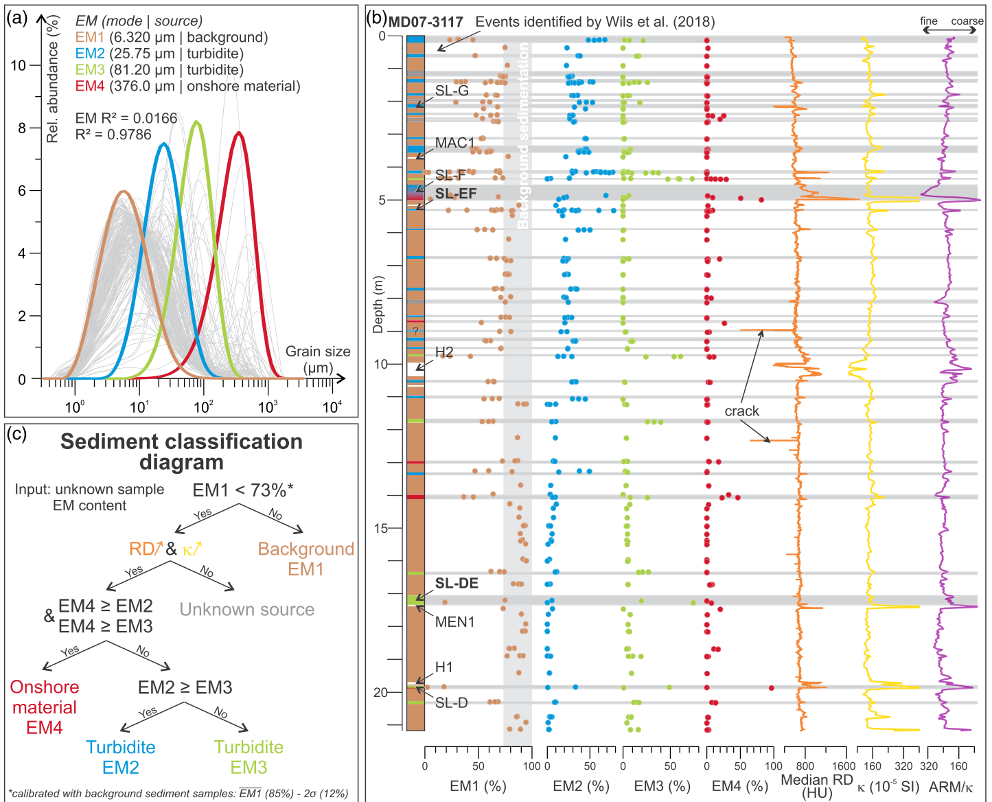
Figure 3. Identification of turbidites in the MD07-3117 sediment core. (a) Grain size results of each of the potential turbidites (gray) is unimixed into four unimodal end-members (EMs)—EM1 (brown, background sedimentation), EM2 (blue, fine-grained turbidite), EM3 (green, coarser-grained turbidite), and EM4 (red, deposition of onshore clastic material). (b) Abundances of each end-member in the different sediment samples, together with the median radiodensity (RD), expressed in Hounsfield Units (HUs) (orange) and some magnetic properties including the volume low-field magnetic susceptibility ( \kappa , yellow, cut off at 400 \times 10^{-5} SI for ease of presentation) and an indication of magnetite grain size (ARM/ \kappa , purple). Interpretation of each sediment interval is visualized by a color-coded schematic representation of the sediment core. White layers represent tephra layers that were not analyzed for their grain size. Deposits that were already identified by Wils et al. (2018) are also marked, and those that were interpreted as the result of megathrust earthquakes are indicated in bold. (c) Schematic representation of how each sample is interpreted.
