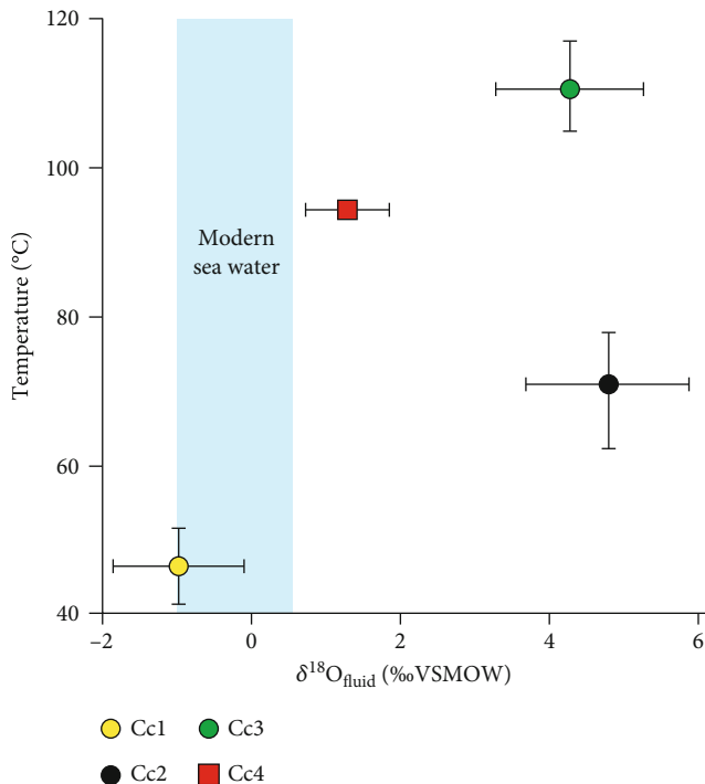
FIGURE 10: Temperatures (°C) vs. \delta^{18}\text{O}_{\text{fluid}} (‰ VSMOW) calculated from clumped isotope thermometry for calcite cements Cc1 to Cc4.
