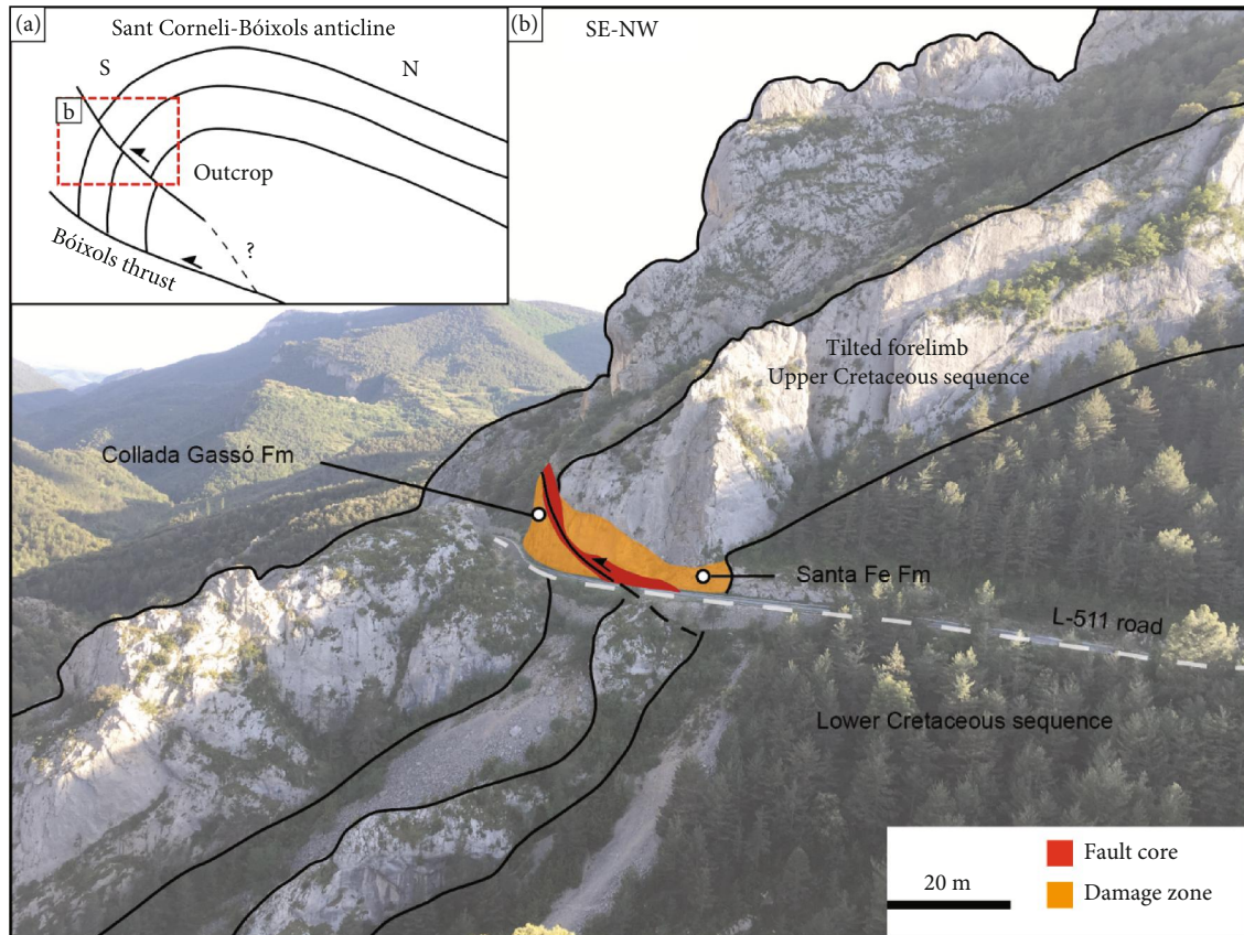
FIGURE 3: (a) Sketch and (b) panoramic view of the studied thrust offsetting the southern limb of the Sant Corneli-Bóixols anticline.
