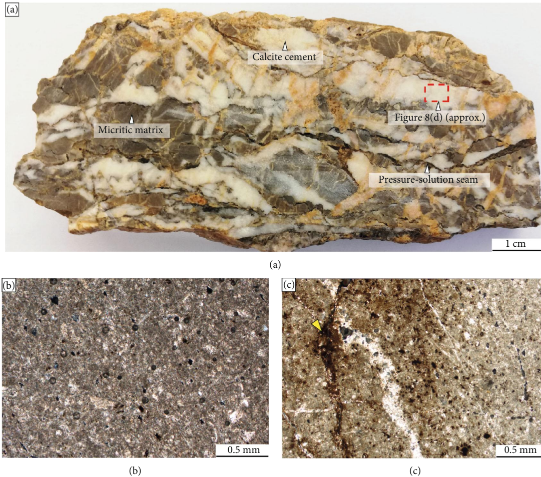
FIGURE 7: Fault core images. (a) Hand sample photograph of the foliated cataclasite showing S-C shear lenses (lithons) of grey host rock micritic limestone and calcite, bounded by dissolution seams or stylolites. Detail of the calcite cement can be found in Figure 8(d). (b, c) Optical microphotographs of the foliated cataclasite matrix with the presence of reddish clay minerals concentrated along pressure solution surfaces (yellow arrow).
