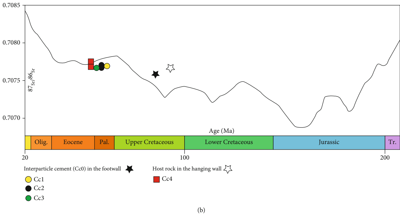
FIGURE 11: (a) ^{87}\text{Sr}/^{86}\text{Sr} isotopic ratios of calcite cements and host carbonates plotted against the Sr content. (b) ^{87}\text{Sr}/^{86}\text{Sr} ratios compared with the ^{87}\text{Sr}/^{86}\text{Sr} isotopic ratios of seawater through time from the LOWESS curve [56].
