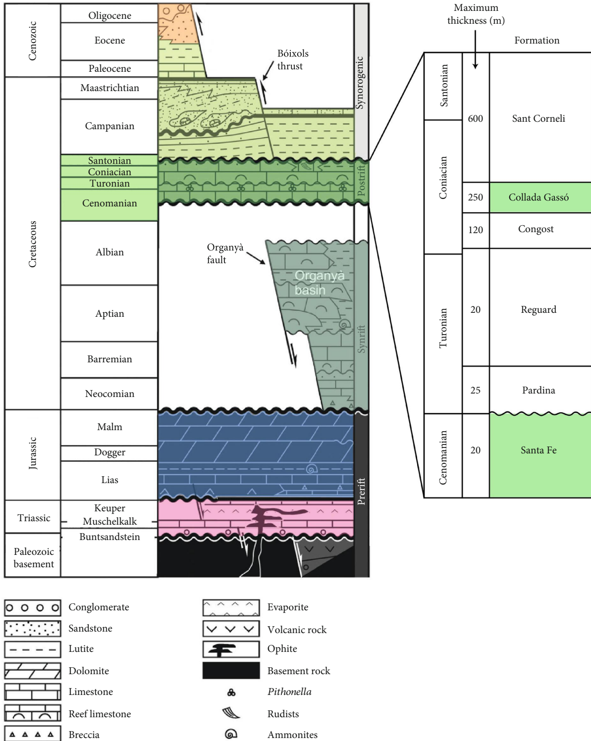
FIGURE 2: Chronostratigraphic diagram showing the main stratigraphic sequences and their related tectonic event [41]. The preorogenic (postrift) sequence, where the thrust was emplaced, is colored in green. The right panel shows a detail of the formations forming this sequence. Thickness and age of these formations are based on [38].
