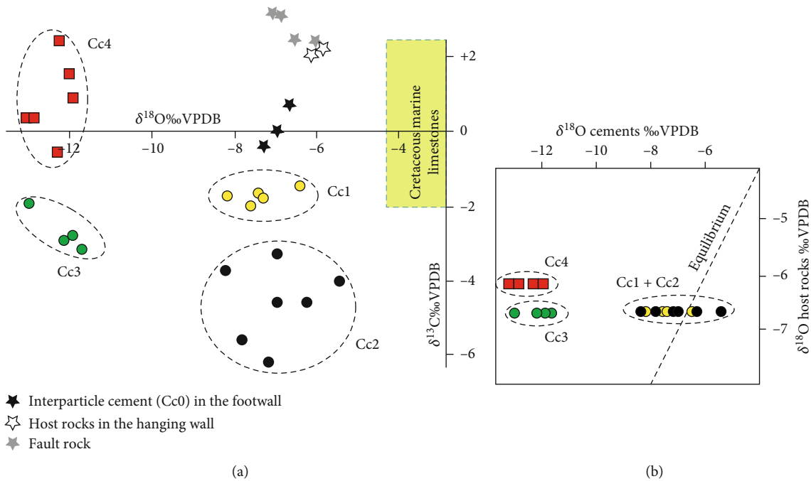
FIGURE 9: (a) Crossplot showing the \delta^{18}\text{O} and \delta^{13}\text{C} compositions of the calcite cements, host rocks, and fault rocks (carbonate matrix from the cataclase). Cretaceous marine limestones values (green box) are from [53]. (b) \delta^{18}\text{O} values of the calcite cements versus \delta^{18}\text{O} values of the related host rocks.
