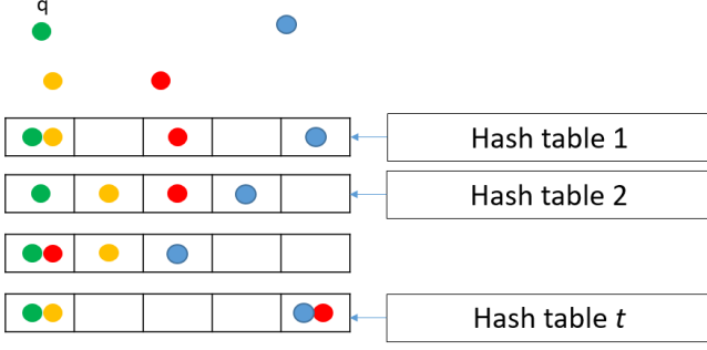
Figure 3. Searching neighbors with the LSH algorithm
