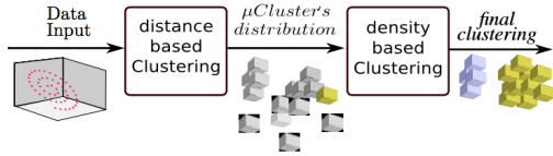
Figure 1. Overview of DyClee
