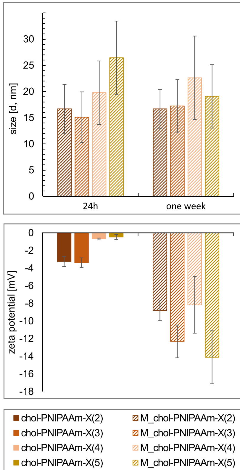
Figure 2 DLS data (size distribution by number) (top), and zeta potential measurement results (bottom).
