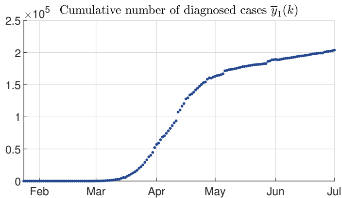
Figure 2: Cumulative number of diagnosed cases \bar{y}_1(k) from January 24 to July 1, 2020. Source: MSS.
