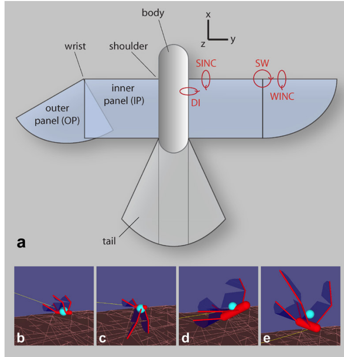
Figure 1 : UAV Morphology. a : Wing panels and their degrees of freedom (DOFs) ; dihedral (DI), sweep (SW), shoulder incidence (SINC) and wrist incidence (WINC). b, c, d, e : four possible morphologies, for extreme values of the wing area ( a_w ) and the wing aspect ratio ( \lambda_w ). UAVs are displayed in flight, with random angular values on the four DOFs. The light-blue sphere indicates the position of the UAV's center of gravity. The yellow line is the trajectory of the UAV's body. b : a_w = 0.1 \text{ m}^2 , \lambda_w = 4.5 , wingspan = 0.67 m. c : a_w = 0.1 \text{ m}^2 , \lambda_w = 10 , wingspan = 1 m. d : a_w = 0.4 \text{ m}^2 , \lambda_w = 4.5 , wingspan = 1.34 m. e : a_w = 0.4 \text{ m}^2 , \lambda_w = 10 , wingspan = 2 m.
