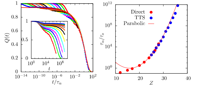
FIG. 5. Extrapolation of the relaxation time in hard sphere simulations using time temperature superposition (TTS) principle in Eq. (9). Left: measured time correlation function Q(t) using either t (inset) and t/\tau_\alpha (main) from Z = 25 to Z = 36 (left to right). The same colors are used in later figures. The full red line is the mastercurve \mathcal{Q}(x) . Right: comparison of measured and extrapolated \tau_\alpha along with the parabolic fit.
