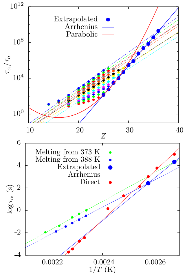
FIG. 6. Extrapolation of the glass melting times (small symbols) in hard sphere simulations (top) and experiments (bottom) on a metallic glass, using Eq. (16) shown as dashed lines. In this figure, symbols with the same colour are obtained by changing T' at constant T with the colour code identical to Fig. 5. For the simulations, the extrapolated data (large blue symbols) fall below the parabolic fit (red line), and are described by an Arrhenius behaviour (blue line). Similar behavior is observed in experiments on a Au-based metallic glass [97], with the extrapolated data falling below the direct measurements.
