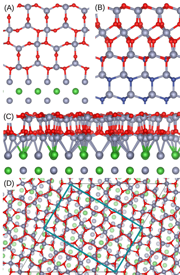
Fig. 9 Atomic structures of supported thin films (colour coding as in Figure 5 and with Ni and N in green and dark blue, respectively). (A): 1 nm thick \theta(100) film on \text{NiAl}(100) ; (B): the native surface oxide on wurtzite- \text{AlN}(0001) (see Ref. 81); (C) and (D): the 5 Å thin \text{Al}_{80}\text{O}_{104} film on \text{NiAl}(110) (see Ref. 27).
