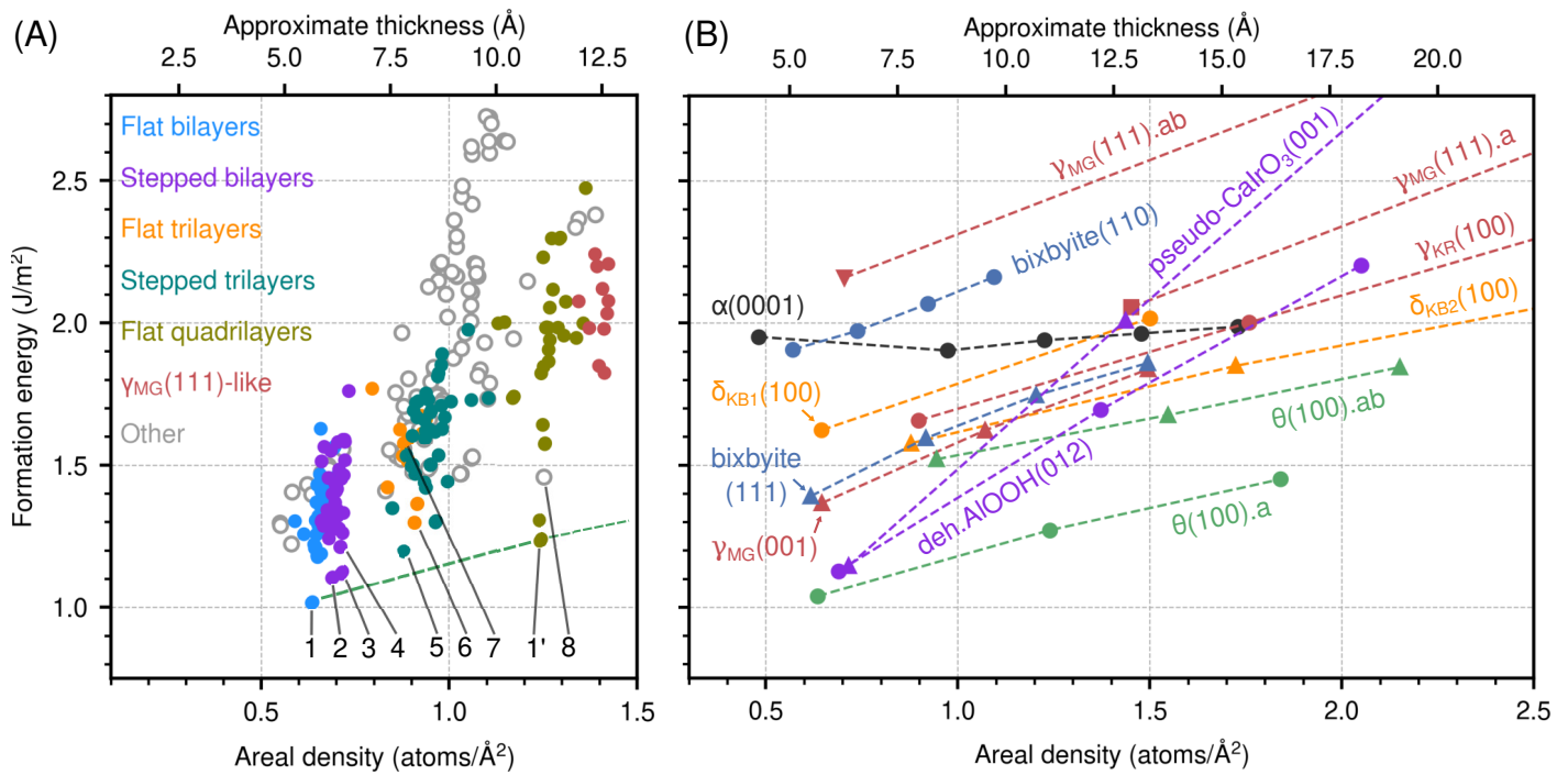
Fig. 2 Calculated formation energies with respect to bulk \alpha - \text{Al}_2\text{O}_3 for the thin films obtained with the 2D-GA (panel A) and by cutting various bulk polymorphs (panel B). Lines are added to guide the eye.
