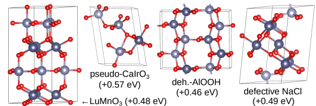
Fig. 4 Structural models and calculated formation energies of the new bulk polymorphs, in eV per formula unit relative to \alpha - \text{Al}_2\text{O}_3 (optB86b-vdW). Colouring as in Figure 3.
