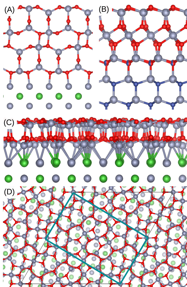
Fig. 9 Atomic structures of supported thin films (colour coding as in Figure 5 and with Ni and N in green and dark blue, respectively). (A): 1 nm thick \theta(100) film on NiAl(100); (B): the native surface oxide on wurtzite-AlN(0001) (see Ref. 81); (C) and (D): the 5 Å thin Al 80 O 104 film on NiAl(110) (see Ref. 27).
