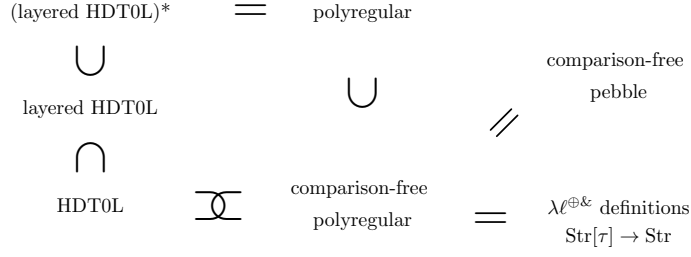
■ Figure 2 Summary of our results. Inclusions \subset where shown to be strict, and \nsubseteq means that there is no inclusion either way. Finally C^* denotes the closure under composition of the class C .
