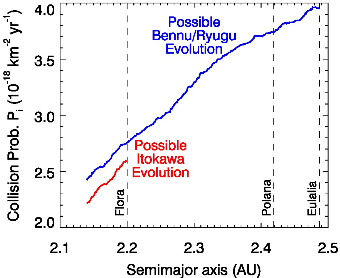
Figure 17. The model collision probabilities of Itokawa, Benu, and Ryugu as they evolved inward toward the Sun across the main belt by the Yarkovsky effect. For Itokawa (red), we assumed that it started at 2.2 au, the center of the Flora family, and then migrated to 2.14 au where it escaped the main belt via the \nu_6 secular resonance. Our Itokawa model asteroids were assigned proper eccentricity and inclination values similar to Gaspra (Table 2). The collision probabilities P_i were calculated with 682 main belt asteroids with D_{\text{ast}} > 50 km (Sec. 2.6). The mean values of all red points are P_i = 2.401 (\pm 0.11) \times 10^{-18} \text{ km}^{-2} \text{ yr}^{-1} and V_{\text{imp}} = 4.98 (\pm 0.04) \text{ km s}^{-1} . For Benu and Ryugu (blue), we assumed that they started at 2.487 au and 2.4 au, the centers of the Eulalia and New Polana families, respectively. The model asteroids were given eccentricities and inclinations of 0.1 and 3^\circ , respectively. The rest of the method was same as with Itokawa. The mean P_i value for Benu and Ryugu starting in the either Eulalia and New Polana families was (3.3 \pm 0.46) \times 10^{-18} \text{ km}^{-2} \text{ yr}^{-1} and (3.1 \pm 0.39) \times 10^{-18} \text{ km}^{-2} \text{ yr}^{-1} , respectively, and their mean impact velocities V_{\text{imp}} were 4.72 (\pm 0.10) \text{ km s}^{-1} and 4.67 (\pm 0.12) \text{ km s}^{-1} , respectively.
