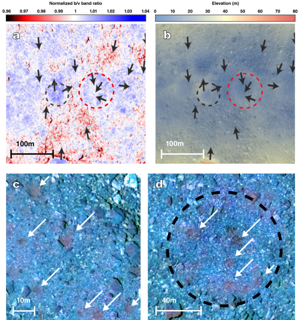
Fig. 4. Examples of crater color. (A) The b/v band ratio map of equatorial craters at 3.05^{\circ}\text{S} , 128.79^{\circ}\text{E} (black dashed line) and 1.06^{\circ}\text{S} , 152.75^{\circ}\text{E} (red dashed line), which have a higher near-UV index and are considered blue units. (B) An elevation map of the same equatorial craters in (A). These blue units correspond with areas that show recent indications of mass movement away from regionally high elevations, such as from crater rims. Black arrows correspond locations of previously mapped mass movement (43). (C and D) RGB color composites images of small craters (indicated by white arrows), shown on the same color scale as Fig. 1A. As indicated by their color, these craters are consistently redder than Bennu's average terrain, with positive to slightly blue b' to x spectral slopes. The blue crater indicated by the dashed black line in (A), (B), and (D) has been overprinted by several smaller reddish craters.
