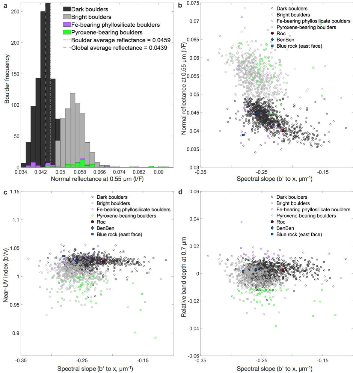
Fig. 2. Variation of boulder color and reflectance on Bennu. (A) Reflectance distribution of boulders ( >5 m) on Bennu. The distribution is multi-modal with more than one Gaussian component (31). Shading and colors indicate different classifications of boulders, as indicated in the legend. (B) Normal reflectance versus absolute spectral slope of the same boulder populations; some individual boulders are indicated in the legend. Dark boulders tend to be redder, and their reflectance monotonically decreases with increasing (redder) spectral slopes, whereas bright boulders are bluer and more scattered (31). (C) The near-UV index ( b'/v band ratio) versus the b' to x spectral slope. Dark boulders tend to have a steeper near-UV slope relative to the global average ( >1 ), whereas bright boulders are more often spectrally flat or show a downturn in the near-UV (from the b' to v bands). (D) The relative band depth at 0.7 \mu\text{m} ( w band) versus the b' to x spectral slope. Some boulders show an absorption feature at 0.7 \mu\text{m} (relative w band depth >0 ), indicative of Fe-bearing phyllosilicates. The boulders named Roc (23.6°S, 25.3°E; Fig. 3C) and
