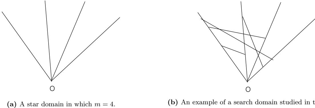
Figure 1: An illustration of different search domains.
