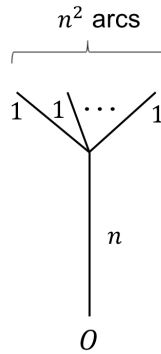
Figure 2: A network for which \rho \approx \sigma/2 .
