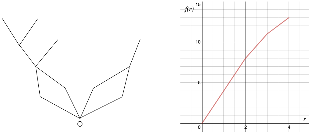
Figure 3: An example of a network Q (left) and the function r \mapsto f(r) \equiv f_Q(r) (right). All arcs in Q are unit-length.
