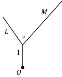
Figure 4: The Y -network.
