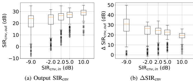
Fig. 12. Influence of the input SIR on the performance of Tango in terms of SIR_{cnv} and \Delta SIR_{cnv} .
