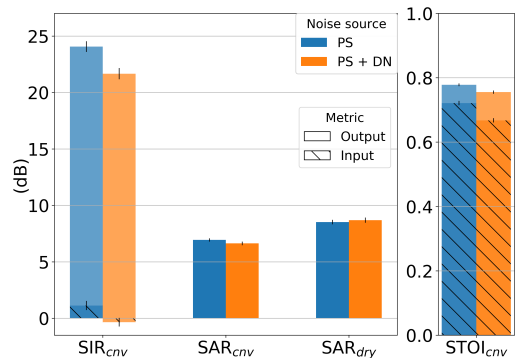
Fig. 10. Speech enhancement performance of the Tango algorithm in the random room configuration when diffuse noise is added to the point noise source. ‘‘PS’’ and ‘‘DN’’ respectively refer to a point source and diffuse noise.
