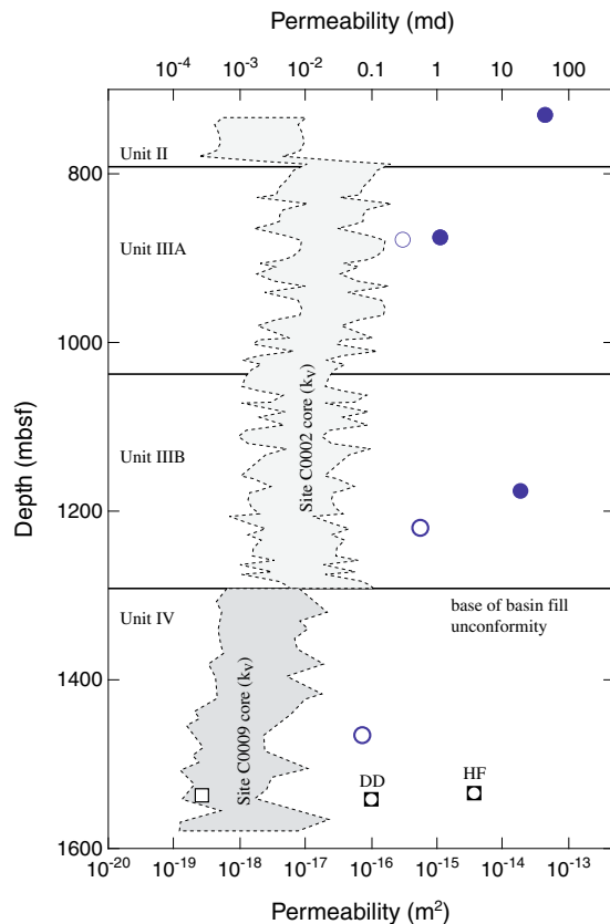
Figure 8. Permeability as a function of depth, reported in \text{m}^2 (lower axis) and millidarcies (top axis). Single-probe (SP) MDT results (blue solid circles = permeability values \geq 10^{-15} \text{ m}^2 ; open circles = values < 10^{-15} \text{ m}^2 ) are computed from equation (1), using the appropriate viscosity for each measurement point based on the in situ temperature estimated from the thermal gradient measured at Site C0002 [Ashi et al., 2009]. As noted in text, SP permeabilities < 10^{-15} \text{ m}^2 may be unreliable. Permeabilities determined by Boutt et al. [2012] from modeling the pressure records for the attempted dual-packer hydraulic-fracture (HF) and dual-packer drawdown test (DD) are shown by partially filled squares. In situ permeabilities are also estimated using porosity from wireline logs at Site C0009, combined with permeability-porosity relationships defined by laboratory tests on core samples (gray-shaded regions). For Units II and III, we use data for data from Site C0002 as an analog (from Guo et al. [2011]) because no cores were collected in these units at Site C0009. For Unit IV, we use experimental data for core samples from Site C0009 ([Boutt et al., 2012] open square; Kitajima et al., unpublished data).
