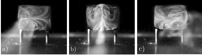
Fig. 3. The bistability : a) Left positioned wake ; b) Transition ; c) Right positioned wake (Grandemange et al. (2012))
