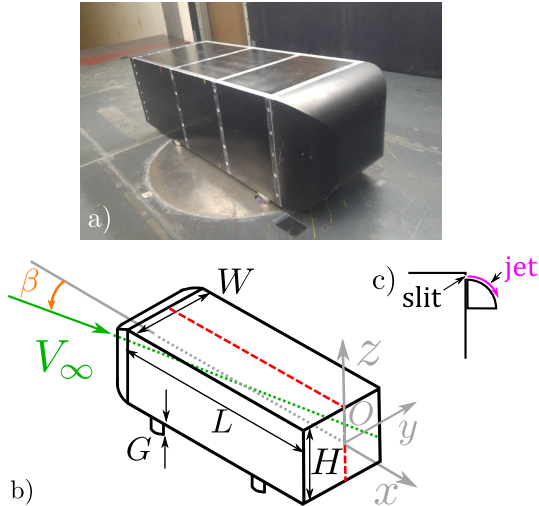
Fig. 1. The experimental mock-up: a) Front view ; b) Back view (schematic) with symmetry plan location (---), the flow velocity direction ( \rightarrow ) and mock-up dimension parameters ; c) Close up view of the Coanda surfaces deviating the actuation jets.
