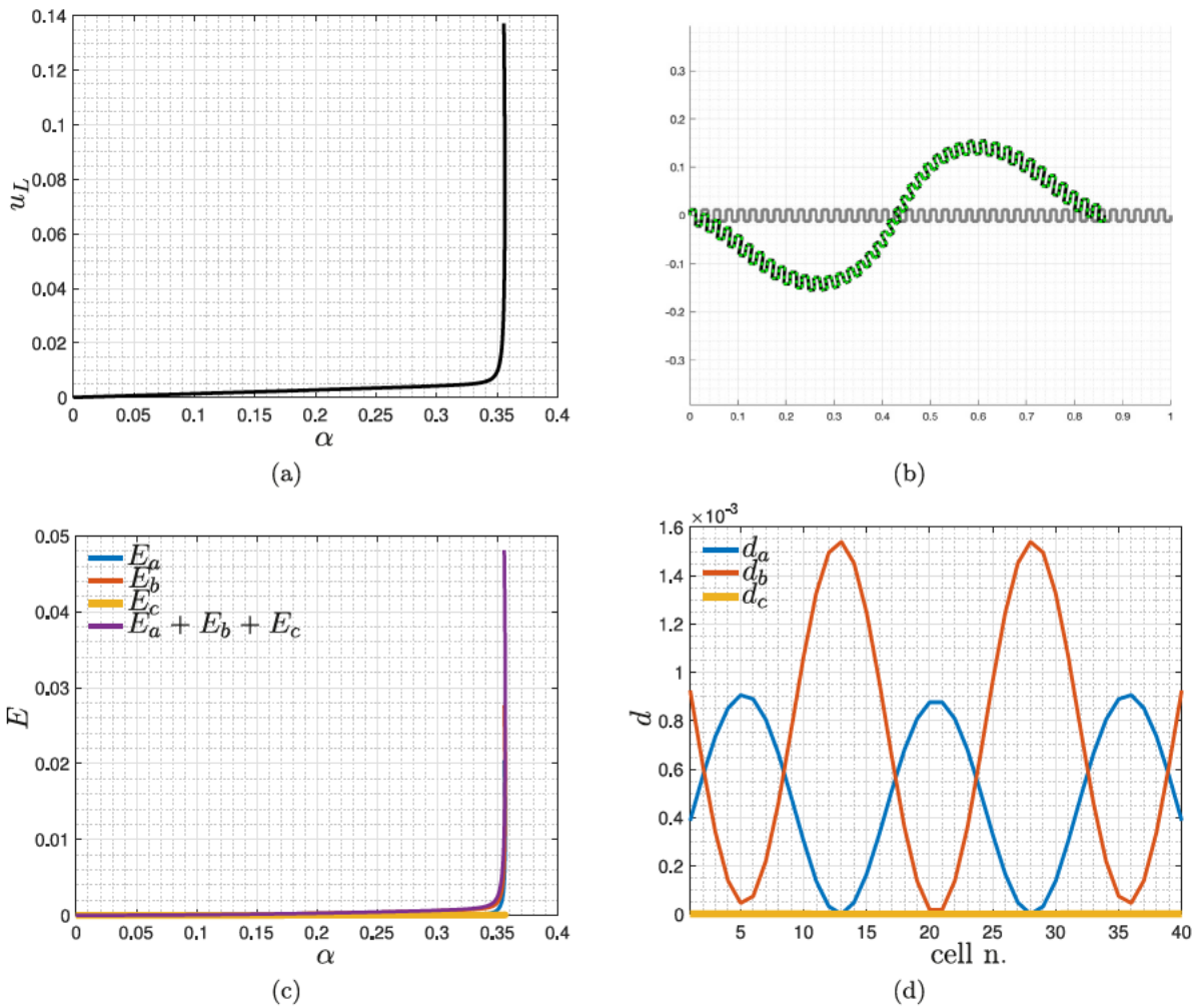
Fig. 22. Duoskelion beam formed by 40 cells subjected to clamp-sliding support kinematic conditions, compression force at the right end-point and modulated transverse perturbation loads at (from the left to the right) 1/4 and 3/4 of the total beam length directed, respectively, downward and upward: equilibrium path (a), final deformation (b), energy evolution (c) and cell energy density (d).
