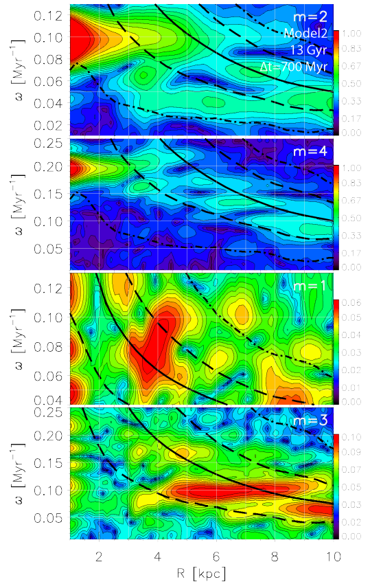
Figure 12. As Fig. 11, but for Model2. As already seen in the TW-method estimates, this bar is about 50% slower than Model1’s bar. Contours in the top two panels are saturated at 1.00 (arbitrary scale in color bar) in order to show the spiral structure better. The reconnection period between the bar and the slower 2-armed spiral is T_{rec} = 2\pi/(2|\omega_b/2 - \omega_{m2}/2|) = 2\pi/|0.1 - 0.04| \approx 105 Myr. The same reconnection periods with the bar are found for both the m = 4 spiral with \omega \approx 0.14 and the m = 3 mode with \omega \approx 0.09 Myr ^{-1} , which can explain the \sim 100 Myr fluctuations of the R_b(t) measurements. As in Model1, m = 2, 3 , and 4 modes conspire to interact with the bar on the same timescale, here \sim 105 Myr, suggesting that we have a strongly coupled system. The longer period of 200 Myr in both R_b(t) and \Omega_p(t) can be related to the faster m = 2 spiral, which has a reconnection period with the bar of T_{rec} \approx 210 Myr. Even longer reconnection periods result from the m = 1 mode near R = 4 kpc and the fast feature in m = 3 with \omega \approx 0.165 Myr ^{-1} , which can be linked to the longer timescale seen in the second half of the time period of Model2 and the wave packet of about 200 – 400 Myr found in the TW-method estimated \Omega_p(t) in Fig. 10.
