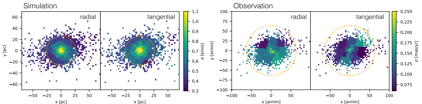
Figure 4. Comparison between velocity dispersion maps of the simulation ( left panel ) and the observation ( right panel ). A higher tangential velocity dispersion is observed along the North-West/South-East direction, in correspondence with the tidal tail overdensities. This feature can be explained by stars in radial orbits preferentially escaping the clusters to form the tidal tails, leaving an overabundance of stars in tangential orbits in proximity of the Lagrangian points. The dashed lines represent the Jacobi radii.
