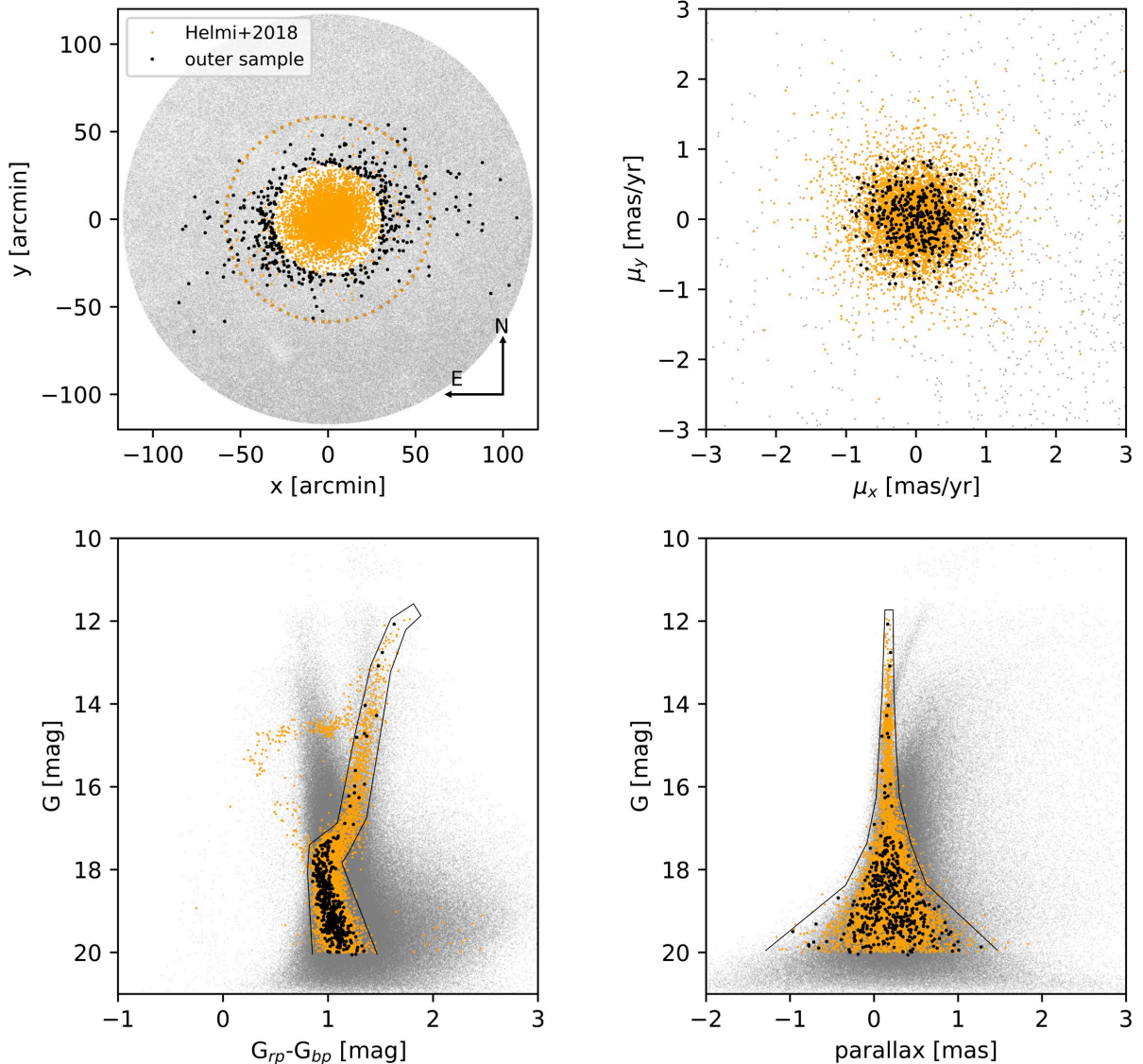
Figure 1. NGC3201 member stars selection in the area extending to 2r_j . The orange points are the inner sample member stars from Gaia Collaboration et al. (2018a) , the grey points all the stars in the 2r_j FoV, and the black dots are the outer stars selected as members in this paper. The membership selection is based on the properties of the \mu_x - \mu_y diagram ( top right plot ), colour-magnitude diagram ( bottom left plot ) and the parallax vs. G magnitude diagram ( bottom right plot ) of the inner sample. Only high-quality proper motion measurements suitable for dynamical analysis are included in the sample. Top left : the FoV of NGC3201 clearly shows the presence of tidal tail structures in the outskirts of the cluster, extending beyond the Jacobi radius (dashed line).
