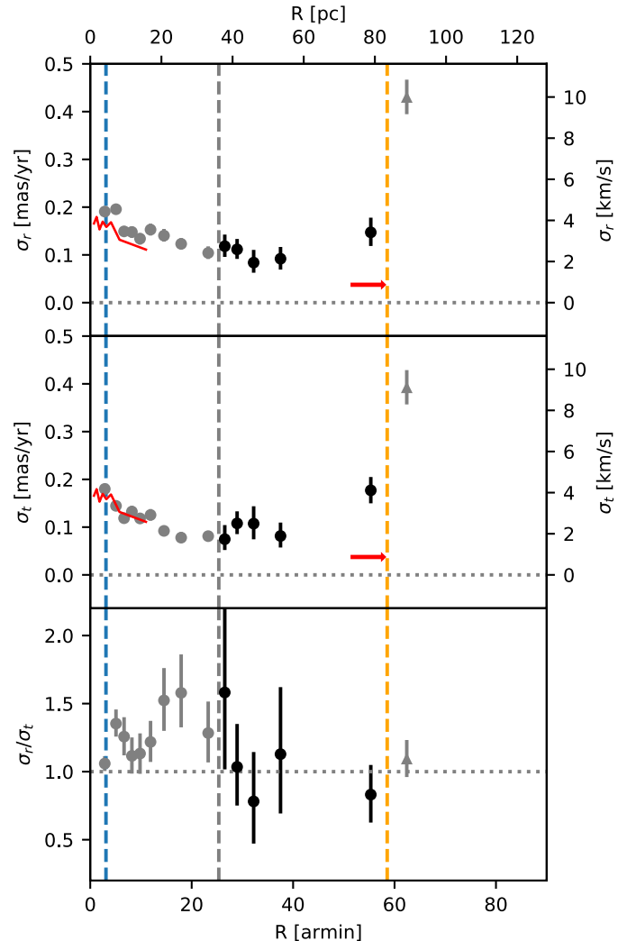
Figure 2. From top to bottom: Velocity dispersion profiles for the radial and tangential component of the proper motions \sigma_r and \sigma_t , and velocity anisotropy profile. Grey circles refer to the region within the tidal radius, while the black circles refer to the outskirts of the cluster; the grey triangles correspond to the values obtained from a looser proper motion cut (see Section 2). The dashed lines are the half-light radius, tidal radius and Jacobi radius, in blue, grey, and orange, respectively. The red line is the line-of-sight velocity dispersion profile from Baumgardt & Hilker (2018) . The velocity dispersion profiles show an evident flattening in the outskirts and higher values than what is expected from the presence of potential escapers only (red arrow, Claydon et al. 2017 ). NGC3201 is radially anisotropic in the intermediate regions and isotropic in the outskirts.
