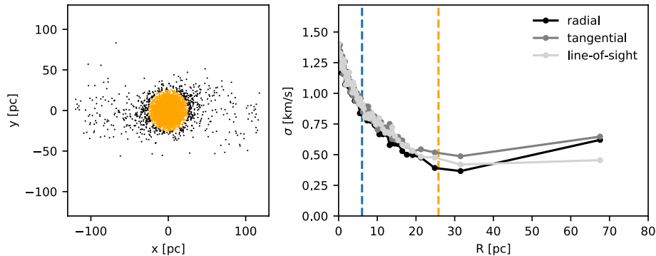
Figure 3. Projected view of a snapshot at 10 Gyr of a N -body simulation forming tidal tails (see Bianchini et al. 2017; Miholics et al. 2016). Orange points indicate stars inside the cluster’s Jacobi radius. The right panel shows that the velocity dispersion profiles of the three velocity components flatten at radii larger than the Jacobi radius (orange dashed line). The blue dashed line is the half-light radius.
