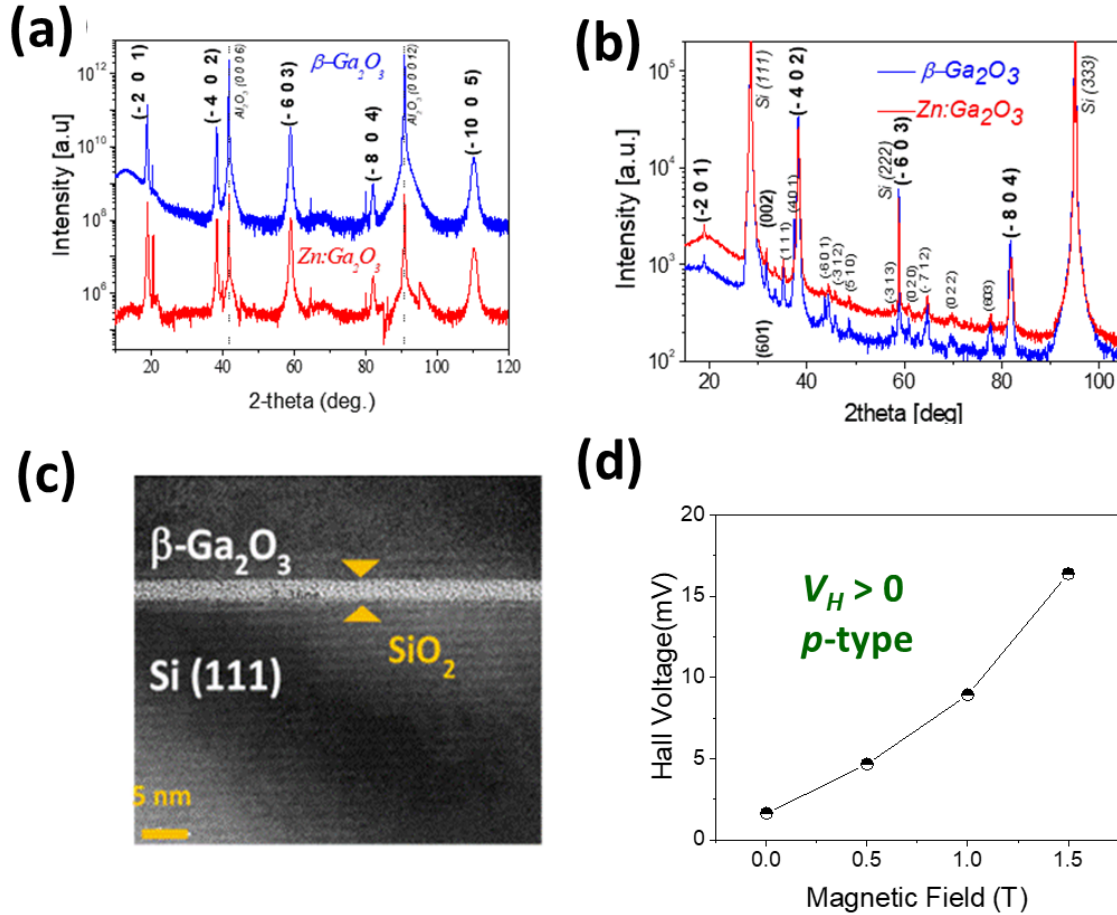
Figure 2: Cu-K \alpha X-ray diffractograms \beta -Ga 2 O 3 and \beta -Zn:Ga 2 O 3 films deposited by MOCVD on (a) Al 2 O 3 (0001) and (b) Si(111) substrates; (c) Transmission electron microscopy of the film on Si(111). Amorphous natural SiO 2 2-3 nm thick layer is evidenced at interface. d) Hall voltage, V_H versus applied magnetic field for T=850K. Positive sign of V_H confirms the p-type conductivity.
