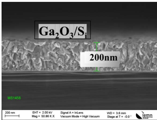
Fig.4 SEM image of cross section for undoped Ga 2 O 3 films grown on Si(111) substrate.
