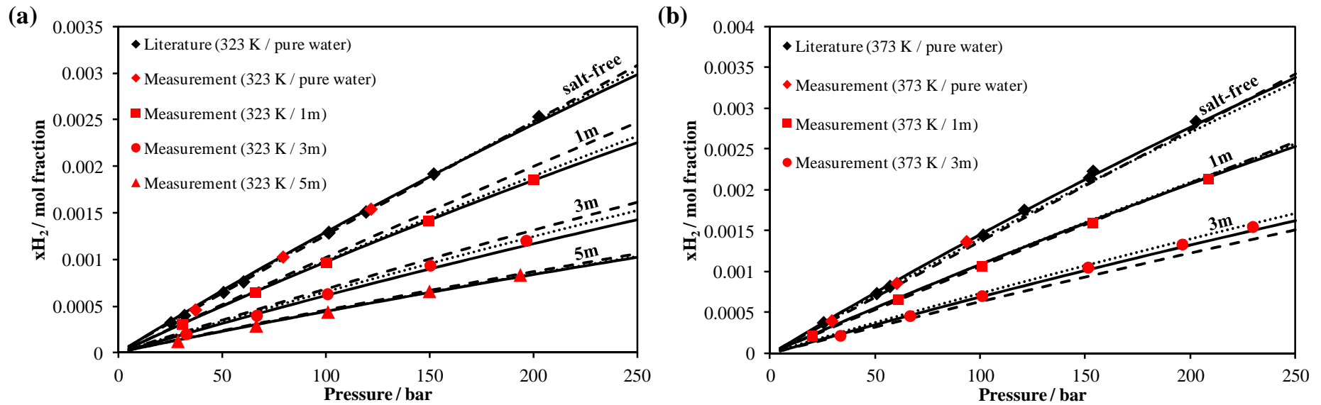
Figure 7 : Solubility of H 2 in H 2 O + NaCl at 323 K (a) and 373 K (b) and different NaCl molalities. Literature data [20, 49, 52] are represented by black symbols and measured ones (Table 4) are represented by red symbols. The solid, dotted and dashed lines represent the H 2 solubilities calculated by the e-PR-CPA, SW, and geochemical models, respectively.
