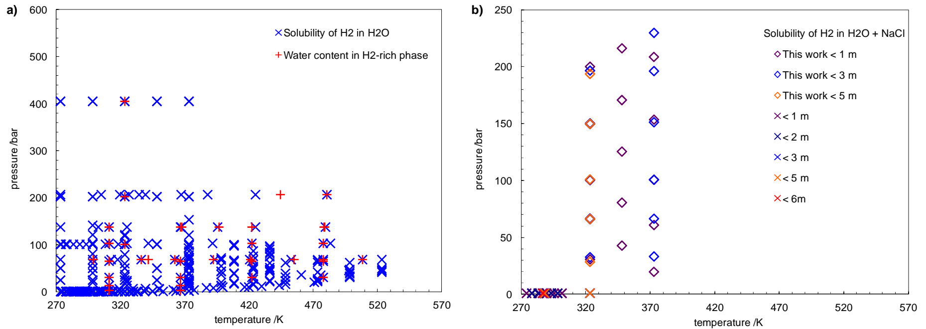
Figure 1 : Distribution of literature solubility data (x) and this work (◇). (a): H 2 -H 2 O system (solubility and water content); (b): H 2 solubility in NaCl brine.
