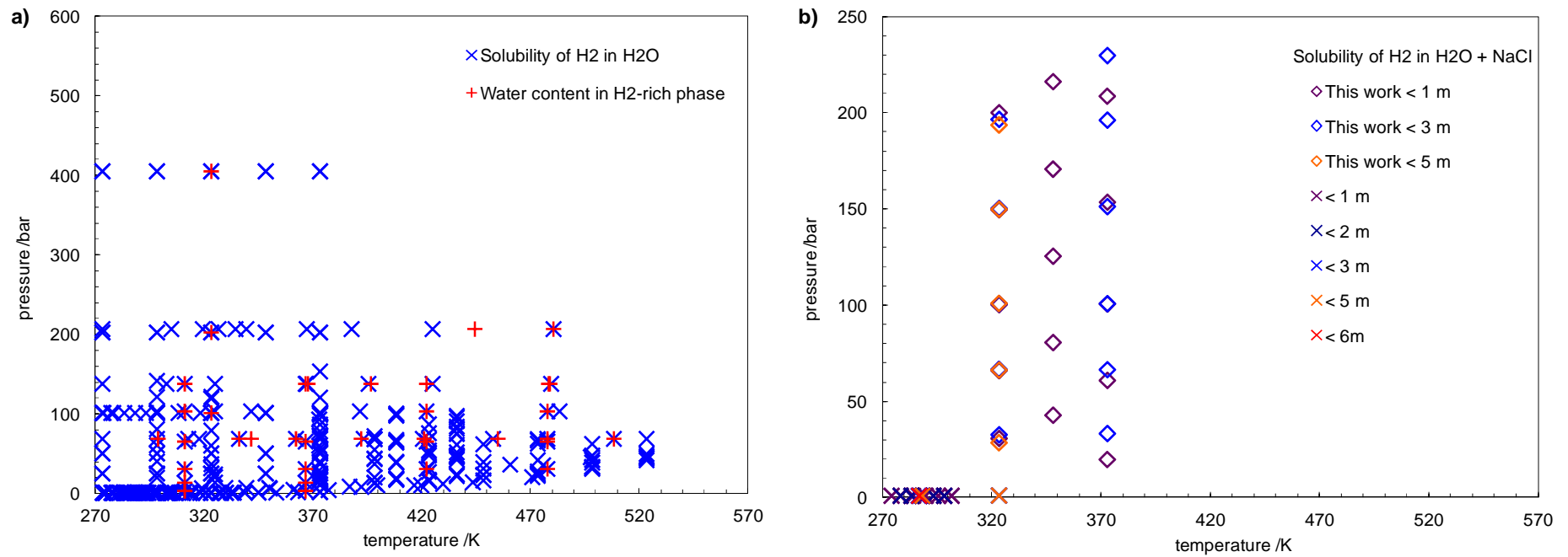
Figure 1 : Distribution of literature solubility data (×) and this work (◇). (a): H 2 -H 2 O system (solubility and water content); (b): H 2 solubility in NaCl brine.
