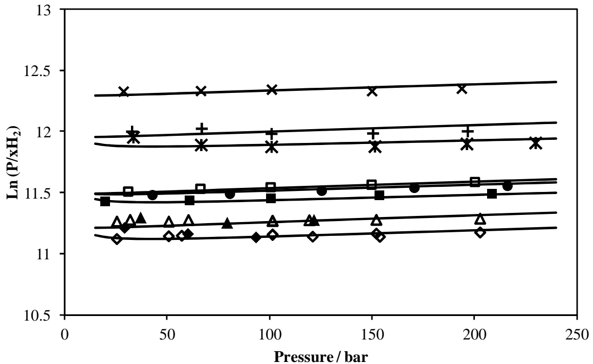
Figure 3: Solubility of H 2 in H 2 O ± NaCl. Literature data [20, 49, 52] are represented by black symbols (Δ: 323 K – pure water; ◇: 373K – pure water) and measured ones (Table 4) are represented by colored symbols (▲: 323 K – pure water; □: 323 K – 1m; +: 323 K – 3m; ×: 323 K – 5m; ●: 348 K – 1m; ◆: 373K – pure water; ■: 373 K – 1m; *: 373 K – 3m). The solid lines represent the predictions of the e-PR-CPA model.
