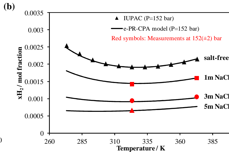
Figure 8 : Effect of temperature, pressure and NaCl concentration (molality) on H 2 solubility. Comparison of literature [20, 49, 52] and some measured (Table 4) data with e-PR-CPA model predictions.
