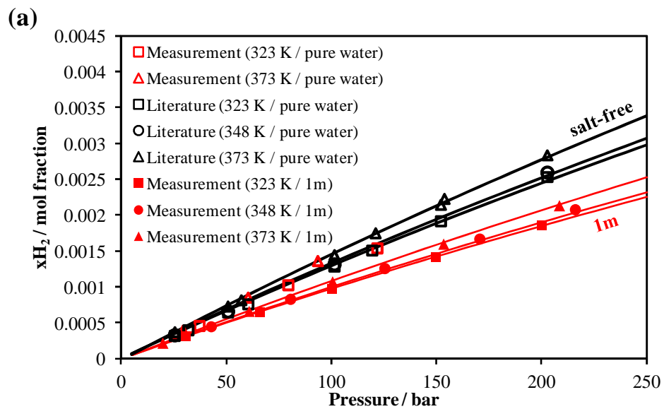
Figure 8 : Effect of temperature, pressure and NaCl concentration (molality) on H 2 solubility. Comparison of literature [20, 49, 52] and some measured (Table 4) data with e-PR-CPA model predictions.
