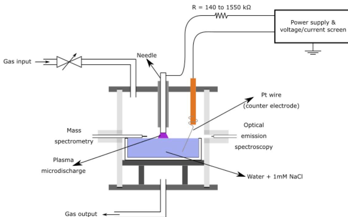
Figure 1: Schematic of the atmospheric pressure DC microplasma experimental set-up.
