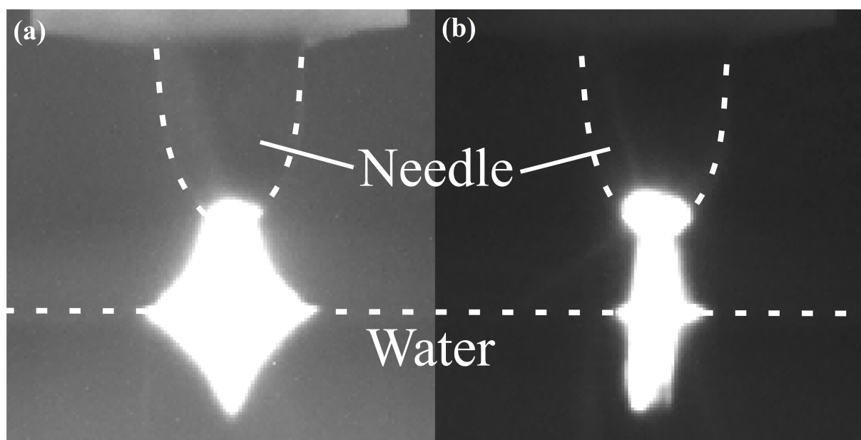
Figure 5: Picture of the plasma when the negative high voltage is applied to (a) the water (water cathode) and (b) the needle (water anode). The plasma is ignited using 730V (2.3kV
