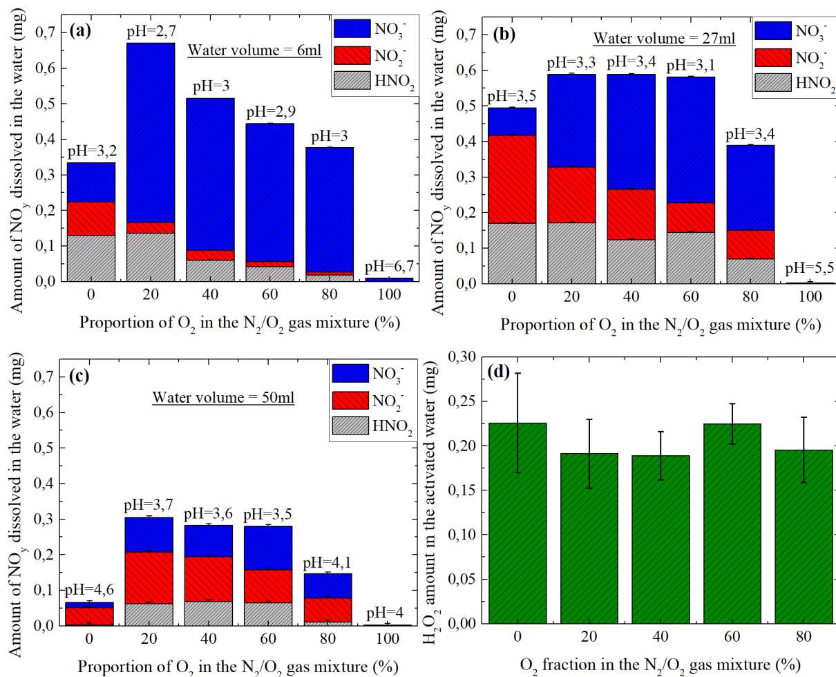
Figure 4: \text{NO}_y measured in the activated water by ionic chromatography following the 12min DC microplasma treatment for different proportions of \text{O}_2 in the gas mixture and for water volumes of 6ml (a), 27ml (b) and 50ml (c) and (d) the corresponding \text{H}_2\text{O}_2 concentration in the solution. The ionic chromatography measurements are performed directly after the plasma is switched off. The discharge is ignited at atmospheric pressure by applying a negative voltage of 730V to the needle (water anode, 2.3kV on the generator, 0.7mm between the needle and the water) and a current of 10mA for 12min. The total gas flow is fixed to 1slm.
