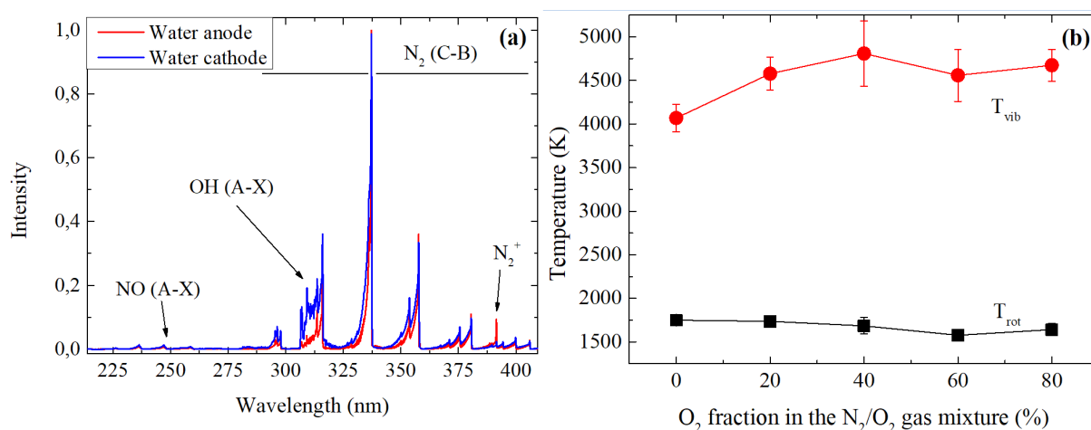
Figure 7: (a) comparison of N 2 microplasmas OES spectra normalized to their highest peak (337nm) in the water cathode and water anode configuration (water tank = 50ml) and (b) rotational and vibrational temperature of plasmas ignited with a water cathode for different oxygen fractions. The plasmas are operated with 730V, 10mA and with a water-needle distance of 0.7mm.
