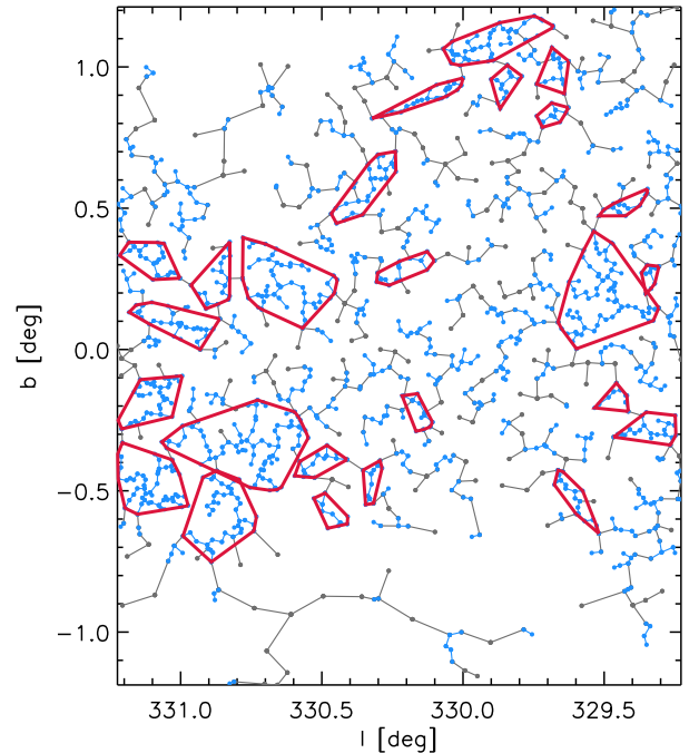
Fig. 4. Result of the MST method applied on the field in Fig. 2. Grey points and lines correspond to \Lambda > \Lambda_{\text{cut}} , whereas blue points and lines correspond to \Lambda < \Lambda_{\text{cut}} . Red lines correspond to convex hulls surrounding groups with N \geq 10 .
