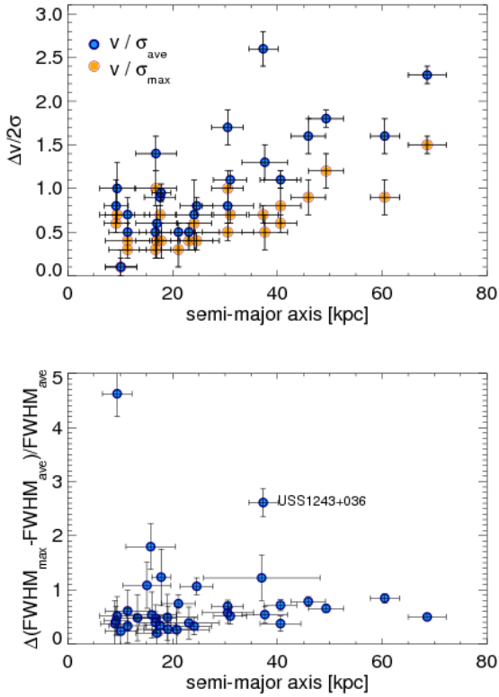
Fig. 12. The ratio of bulk to turbulent velocity (parametrized as \Delta v/2\sigma , see Sect. 7.5) in the 25 sources with extended gas in Table 4 scales with the size of the emission-line region ( top panel ). We plot \Delta v/2 instead of \Delta v , because this gives an approximation to the circular velocity in case of rotationally dominated motion. The offset between maximal and average FWHM does however not depend on the source size ( bottom panel ).
