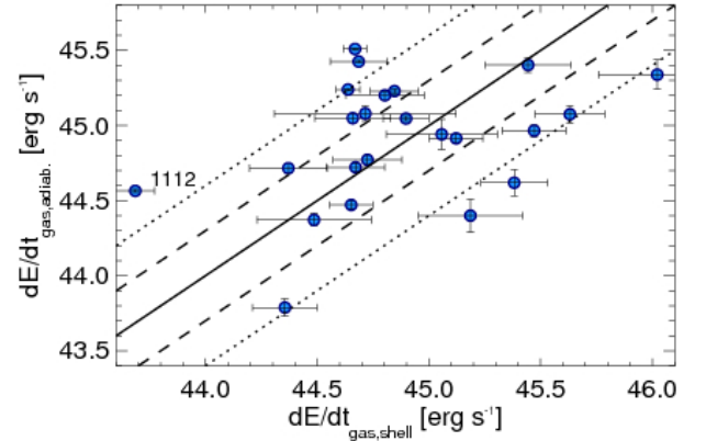
Fig. 18. Comparison of the results of our two kinetic energy estimates in Sect. 7.5 for the 23 galaxies with extended emission line regions, which have been observed in [\text{OIII}]\lambda 5007 . The dashed and dotted lines show offsets by factors 2 and 4, respectively, from the one-to-one relationship (solid line).
