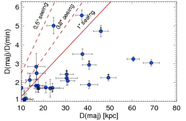
Fig. 3. The ratio between major and minor axis of the extended emission-line regions in our 27 galaxies with well resolved line emission (Table 4), as a function of major axis length. Typical ratios are between 2 and 4. More extended regions are also more elongated.
