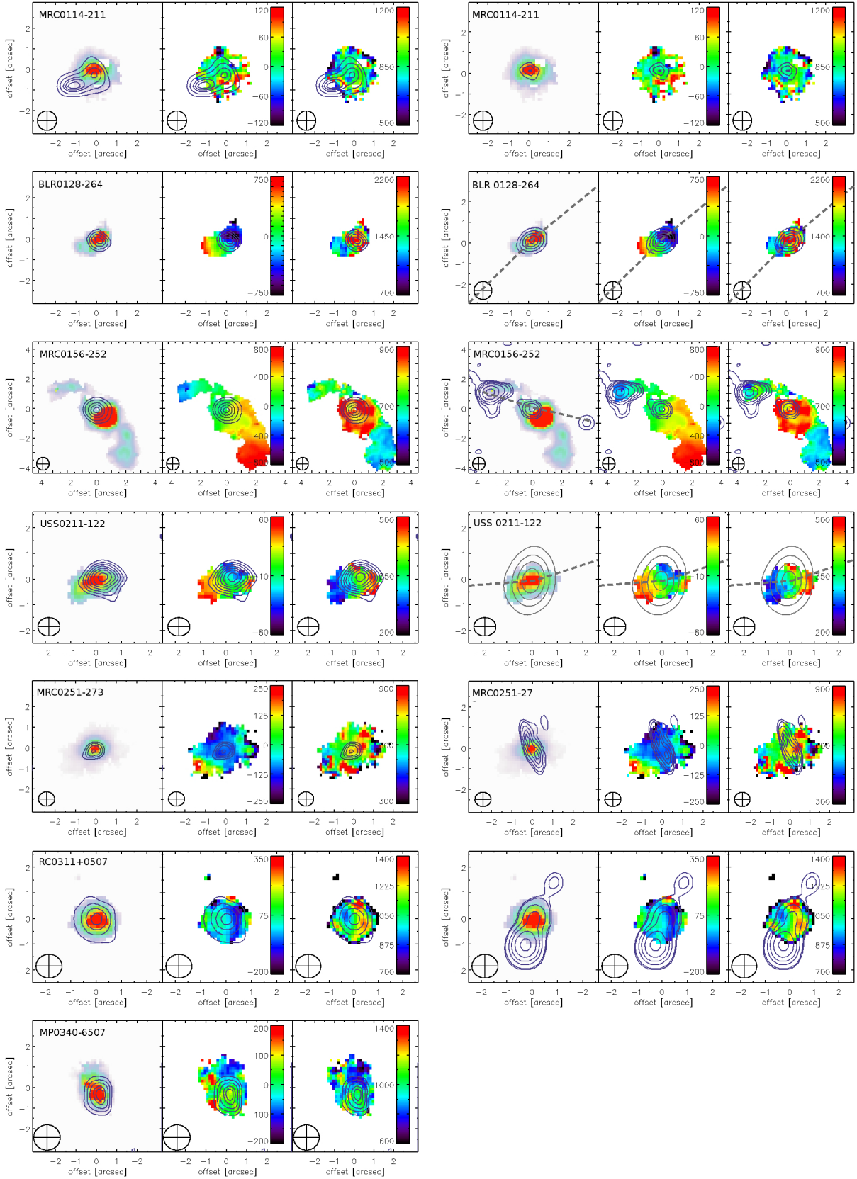
Fig. A.4. Maps of our galaxies in order of RA, with the rest-frame optical continuum shown as contours in the left , and the GHz radio continuum in the right panel . In each panel, maps show (from left to right ) emission-line morphology, velocities relative to the average redshift of all pixels covered by the emission-line region, and FWHM line width. Relative velocities and line widths are given in \text{km s}^{-1} . In galaxies where we did not detect the rest-frame optical continuum, we show the emission-line morphology instead of the optical continuum (with red contours, the continuum is shown as blue contours). Coordinates are given relative to the position listed in Table 1. Contour levels are arbitrary, their main purpose is to guide the eye.
