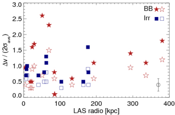
Fig. 13. Ratio of ordered to unordered motion, \Delta v/\sigma , as a function of radio size. We show all 25 sources from Fig. 4 with measurements of \Delta v/\sigma . Filled and empty symbols show the maximal and average line widths, respectively.
