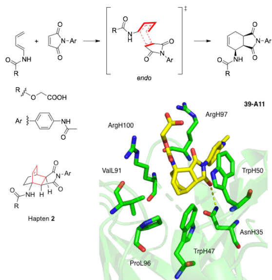
Figure 6. DA reaction catalyzed by antibody 39-A11 raised against the bicyclic haptin 2 and X-ray structure of antibody 39-A11 including the haptin 2 (pdb: 202w). H and L-labels of amino acid residues refer to the heavy and light chains of antibody, respectively.
