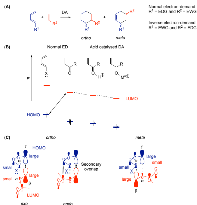
Figure 2. DA reaction (A) Regiochemistry; (B and C) Frontier orbitals HOMO and LUMO involved in normal electron-demand DA reaction ( \ddot{X} = \text{EDG} )
