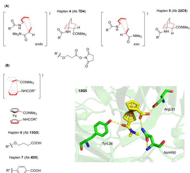
Figure 8. DA reaction of 4-carboxybenzyl trans -1,3-butadiene-1-carbamate and N,N -dimethylacrylamide catalyzed (A) by antibodies 22C8 and 7D4 raised against the bicyclic haptens 4 and 5 ; (B) by antibodies 13G5 and 4D5 raised against ferrocenyl haptens 6 and 7 . RX structure of the 13G5 with the 1-carboxy-1'-[(dimethylamino)carbonyl] inhibitor (pdb: 1a3l).
