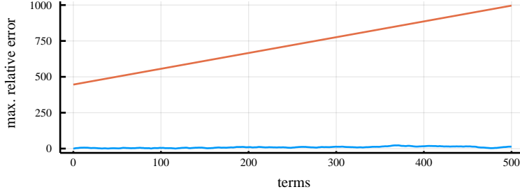
FIGURE 10.1. Bound from Proposition 10.5 (top curve) and measured error (bottom curve), in multiples of the unit roundoff u , for the evaluation of the scaled Bernoulli numbers in 53-bit floating-point arithmetic with unbounded exponents. The script used to produce this plot is available in the supplementary material.
