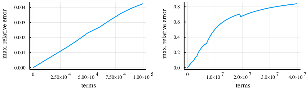
FIGURE 9.1. Measured error in the evaluation of the sequence (c_n) defined by (9.1) in IEEE binary32 floating-point arithmetic ( u = 2^{-24} \simeq 6 \cdot 10^{-8} ). For each n , we plot the maximum observed error on c_n for 997 exactly representable values of c_0 regularly spaced in the interval [\pi/2, \pi] . The script used to produce these plots is available in the supplementary material.
