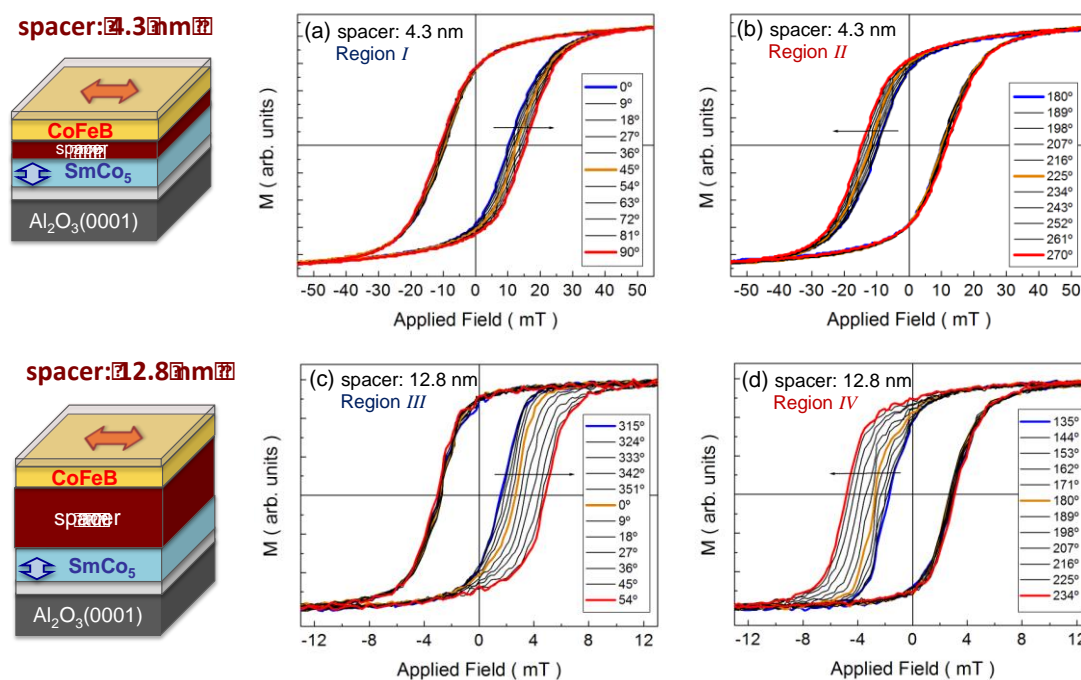
Fig. 4. In-plane hysteresis loops measured by MOKE with magnetic field applied at different in-plane angles, \alpha_H , and corresponding to colored regions I–II and III–IV in Figs. 3a,b, respectively, for: (a) and (b) \text{SmCo}_5(30\text{nm})/\text{spacer}(4.3\text{nm})/\text{CoFeB}(3\text{nm}) ; and (c) and (d) \text{SmCo}_5(30\text{nm})/\text{spacer}(12.8\text{nm})/\text{CoFeB}(3\text{nm}) . \alpha_H = 0^\circ corresponds to application of the external magnetic field parallel to the easy axis direction of the \text{Si}/\text{SiO}_2/\text{CoFeB} reference sample. Arrows are visual guides to show the continuous increase in coercivity when varying \alpha_H while maintaining one of the loop branches pinned.
