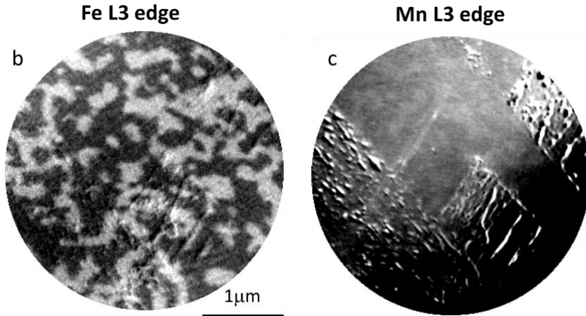
Figure S3 a-b. XMCD-PEEM image measured at zero field and room temperature at the Fe L3 edge (b) and Mn L3 edge (c). The sample is composed of a //Ta(3)Cu(3)/IrMn(5)/Pt(0.5)/Co(0.3)/NiFe(0.59)/Al(2) (thickness in nm) multilayer deposited by magnetron sputtering on a Si wafer. The sample was heated above the blocking temperature of the AFM (at 250°C for 30 minutes) and then cooled in a large external magnetic field (0.57 T) applied perpendicularly to the film plane.
