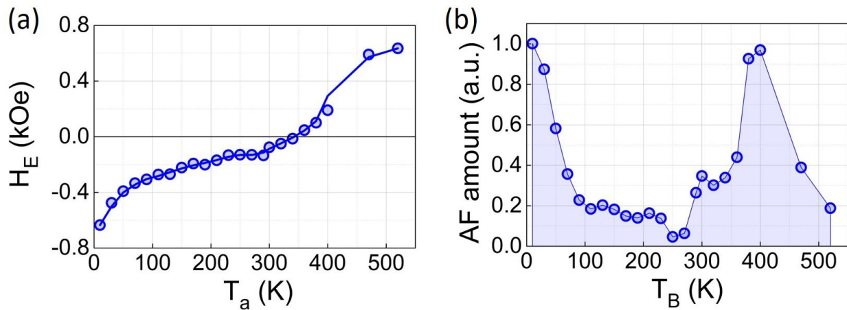
Figure S4 (a) Variation of H_E vs. T_a for a //Ta(3)/Cu(3)/IrMn(5)/Pt(0.5)/Co(0.3)/NiFe(0.87)/Al(2) (nm) multilayer. The full line is a smooth interpolation of the data. (b) Blocking temperature distribution, corresponding to the derivative dH_E/dT_a vs. T_a from the data interpolation.
