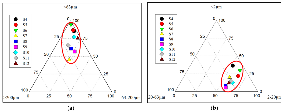
Figure 2. Ternary textural diagrams of bottom sediments of the Lomé lagoon: (a) for the total fractions (<2 mm), (b) for the fine fractions (<63 \mu\text{m} ). S4 to S12 are the different sampling stations (see locations in Figure 1).
