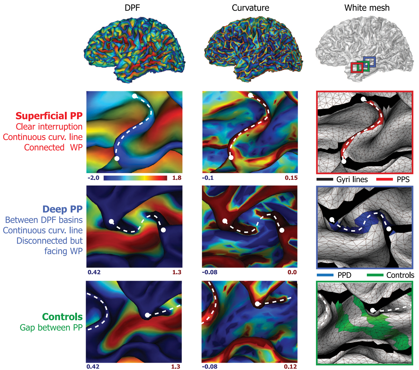
Fig. 3. Methods for PPs identification, illustrated for one subject in the left hemisphere. Top panel: Surface maps generated in BrainVisa and projected on the white matter surface. DPF map shows an increasing depth from blue to red color. Curvature (finite element method) map shows an increasing curvature from blue to red color. Squared panels: Morphological criteria used to characterize PPs (represented by white dotted lines). Zoom windows illustrate the manual identification of one example superficial PPS (first row) and deep PP (PPD, second row) as well as controls (third row) generated automatically. Once detected based on the morphological criteria (written on the left), PPs are drawn by selecting the intersections (white dots) between their two extremities and the adjacent gyri crests (in black). A line is then automatically generated between this pair of vertices passing by the shortest path and constrained by minimal DPF values (Le Troter et al., 2012). Controls are generated using a similar procedure except that their position is generated automatically into the sections separating PPs locations. If there is enough space, several controls are generated with different orientations. Here, two controls (in green) were generated between two true PPs (white dotted lines). Numbers under the squared panels indicate the range of the blue-to-red colormap used to generate the respective figures. DPF: Depth Potential Function; PP: plis de passage; WP: wall pinches.
