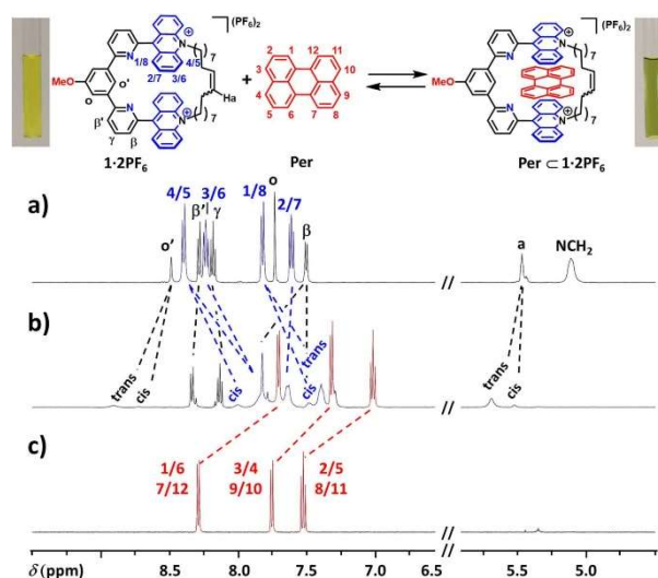
Figure 2. ^1\text{H} NMR (500 MHz, \text{CD}_3\text{CN} , 298 K, c = 1.5 \times 10^{-3} \text{ mol L}^{-1} ) spectra of (a) 1-2PF 6 , (b) the 1:1 mixture of Per and 1-2PF 6 , and (c) Per . The photographs of the solution of 1-2PF 6 and the 1:1 mixture of Per and 1-2PF 6 are shown.
