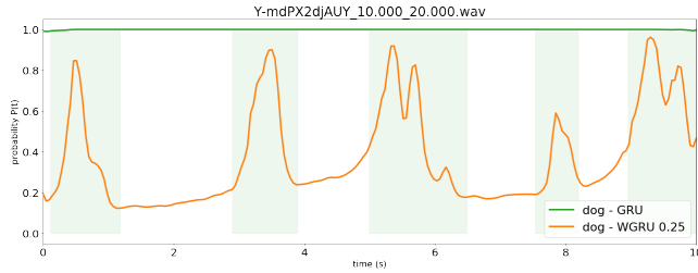
Figure 2: GRU (green) and WGRU (orange) score curves for the correct class Dog . The vertical rectangles denote the groundtruth and represent the segments where Dog should be detected. Green Localization results of the CRNN with GRU. The class dog is detected but in the entire clip. Orange : The prediction of the CRNN with WGRU with a temporal weight of 0.25. The dog barking segments are detected and localized properly.
