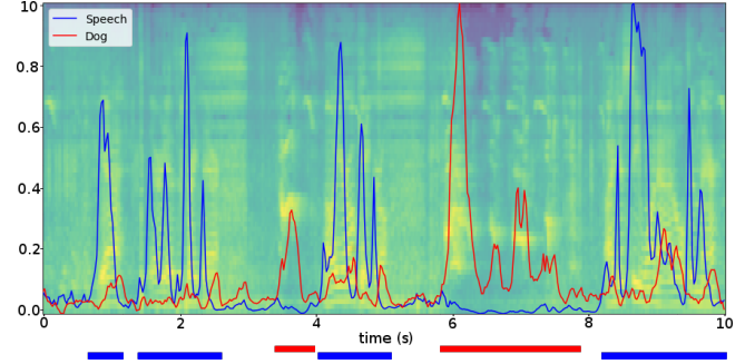
Figure 3: Score curves by MIL for the two correctly detected classes 'Speech' (Blue) and 'Dog' (Red). Below the spectrogram is represented the groundtruth.
