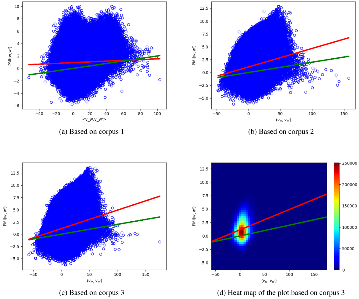
Fig. 3: Experiments on equation 10. x-axis: \langle v_w, v_{w'} \rangle ; y-axis: PMI(w, w') . Green line: theoretical linear relationship predicted by the equation. Red line: result of the linear regression.
