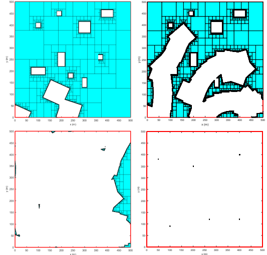
Fig. 3. Initial \overline{\mathbb{Z}}_1 (top left), \overline{\mathbb{Z}}_{15} (top right), \overline{\mathbb{Z}}_{100} (bottom left), and \mathcal{Z}_{100} (bottom right)
