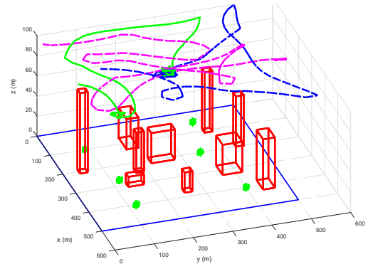
Fig. 4. Resulting trajectories for 3 UAVs; targets (static): green stars; obstacles: red polyhedrons
