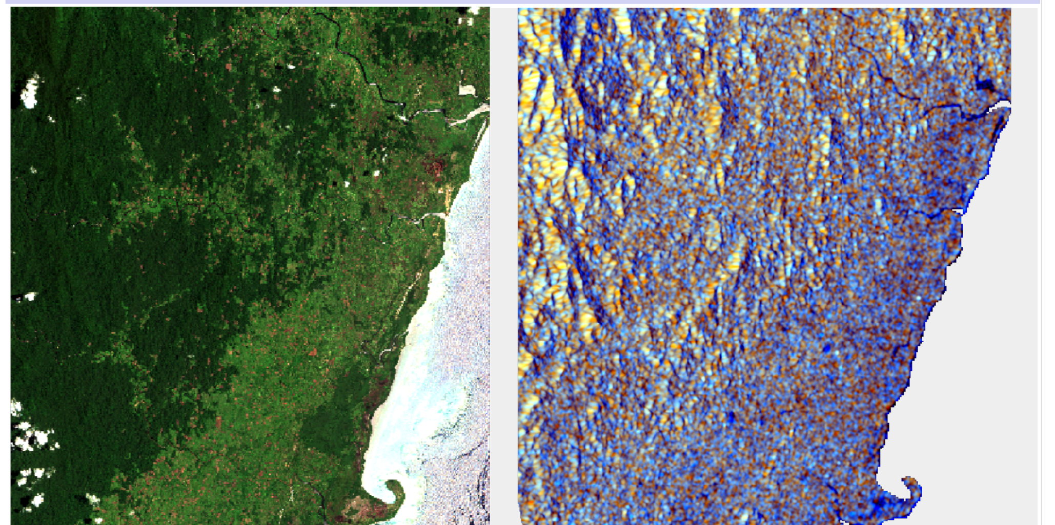
Sentinel 2 image
