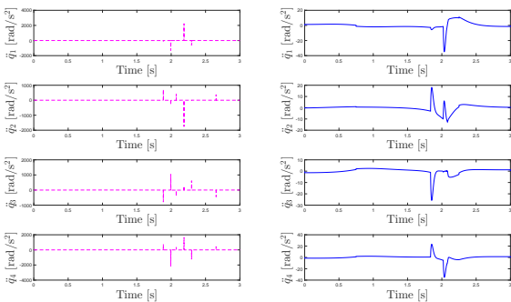
Fig. 4. Comparison between the joint accelerations given by the local-QP (dashed magenta) and the proposed (solid blue) methods in the constrained case ( k = 2 ). Note the different axis scales.
