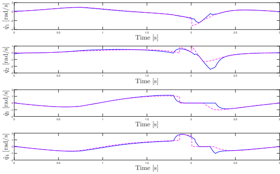
Fig. 2. Comparison between the joint velocities given by the local-QP (dashed magenta) and the proposed (solid blue) methods in the constrained case ( k = 1 ).
