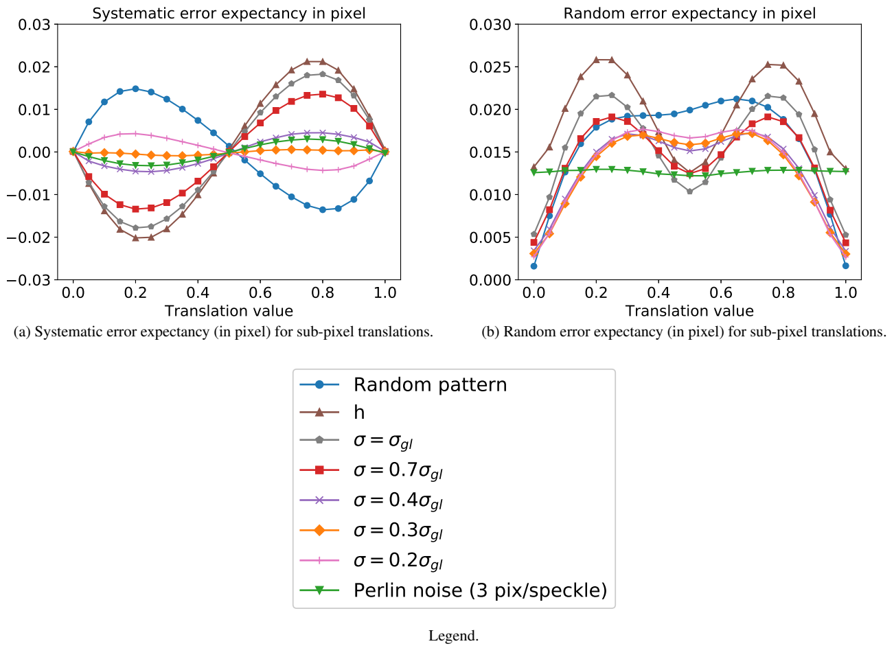
Fig. 5: Systematic and random error expectancies for sub-pixel translations. Results are presented for the random pattern, the initial pattern h , F_{\mu,\sigma}(h) for five different values of \sigma ranging from 0.2\sigma_{gl} to \sigma_{gl} , and the Perlin noise pattern.
