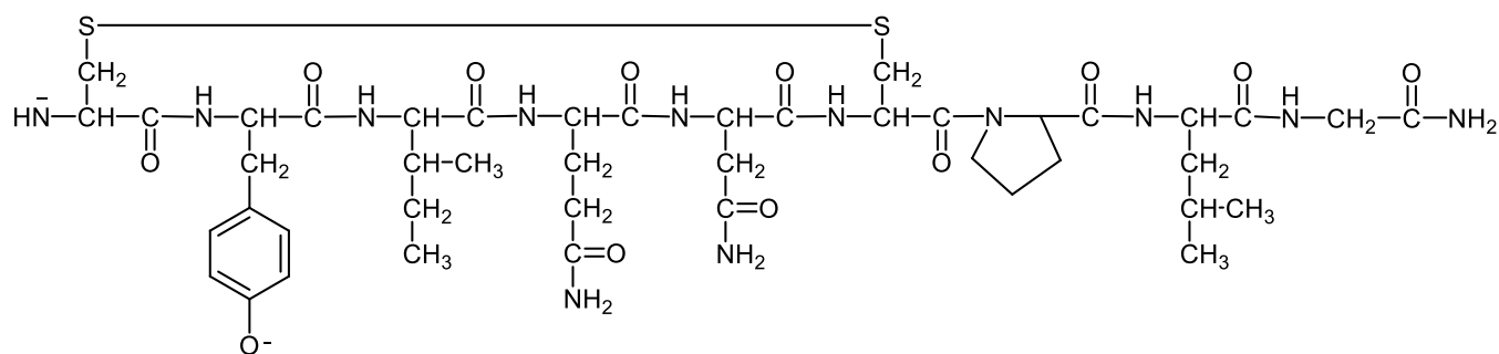
Scheme 2 : Proposed structure for [OT-2H]^{2-} .
