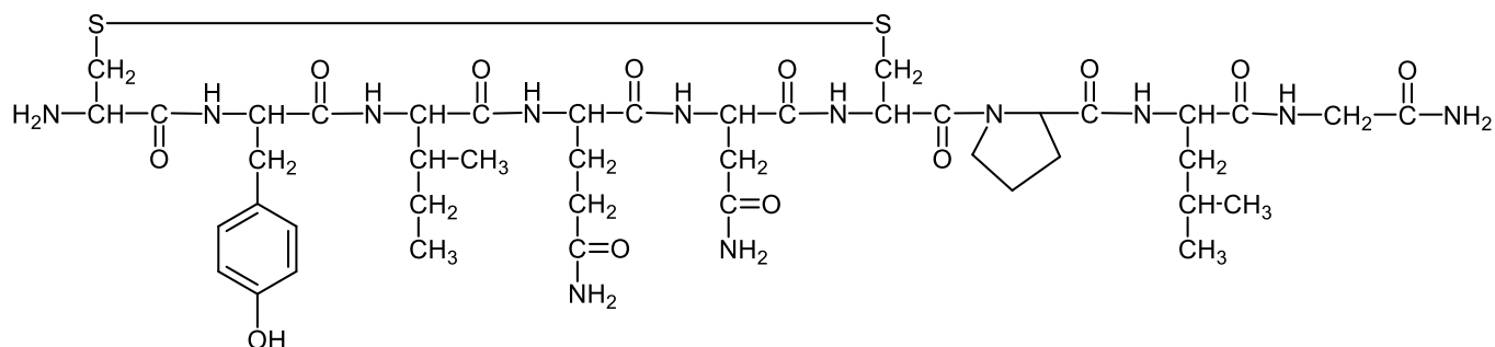
Scheme 1 : Chemical structure of oxytocin
