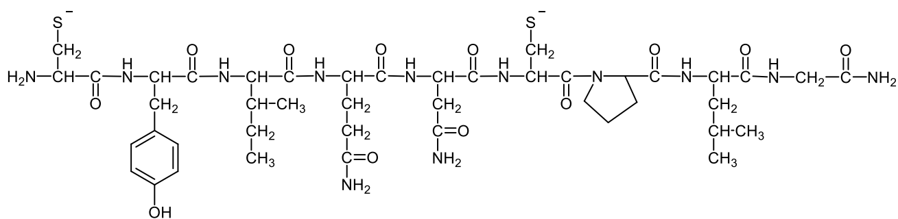
Scheme 3 : Proposed structure for [OT^{SH}-2H]^{2-} .
