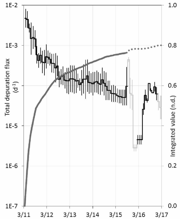
Figure 7. Time evolution of the mean total activity depuration flux derived from data ( GM \pm GSD ) and its cumulated value ( GM ), with the assumption that f=0.85 for KAJI sites. The grey portions indicate periods when throughfall or litterfall are missing.
