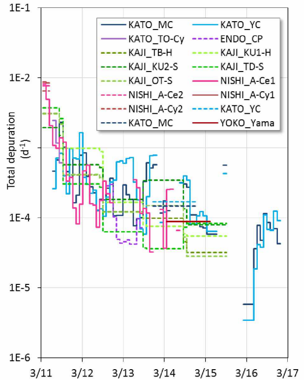
Figure 3. Time evolution of the site-specific activity depuration flux (14 sites), with the assumption that f=0.85 for KAJI sites.
