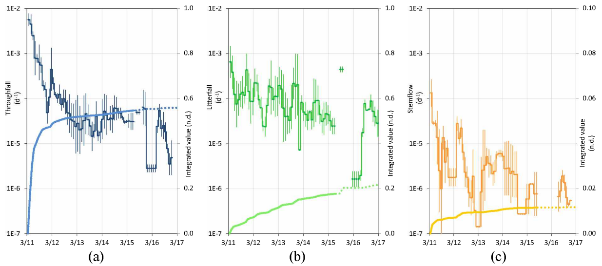
Figure 8. Time evolution of the mean activity depuration fluxes derived from data ( GM \pm GSD ) and their cumulated values (GM): (a) throughfall, (b) litterfall and (c) stemflow. The dotted lines have been calculated by assuming that fluxes were nil in the absence of measurements.
