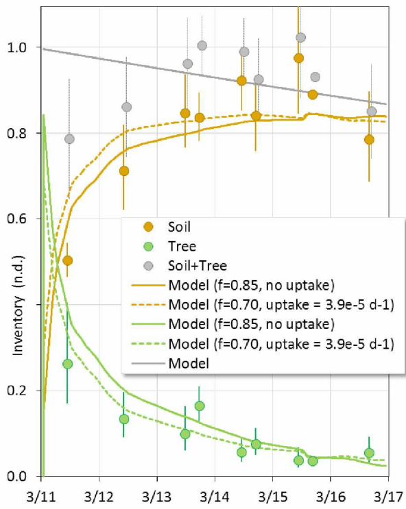
Figure 6. Time evolution of the mean activity inventories in soil and tree vegetation derived from data ( GM \pm GSD ) and predicted by the compartmental model with f=0.70 and 0.85 .
