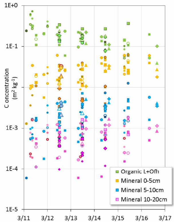
Figure 5. Time evolution of the site-specific activity concentrations in the organic and mineral soil layers (23 sites, about 4 \times 80 data). GSDs are not displayed for graphical reasons.
