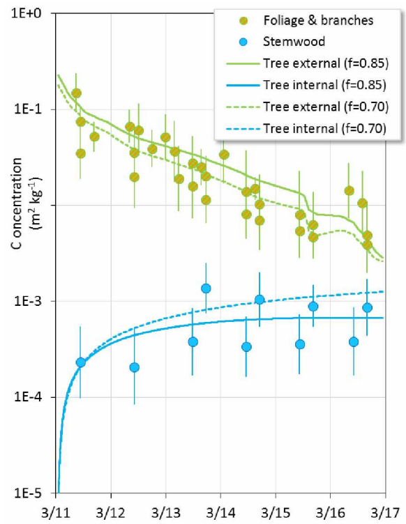
Figure 10. Time evolution of the activity concentrations in tree external and internal organs predicted by the compartmental model with f=0.70 and 0.85 (best estimates).
