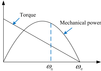
Fig. 2. Simplified linear torque model [1]
