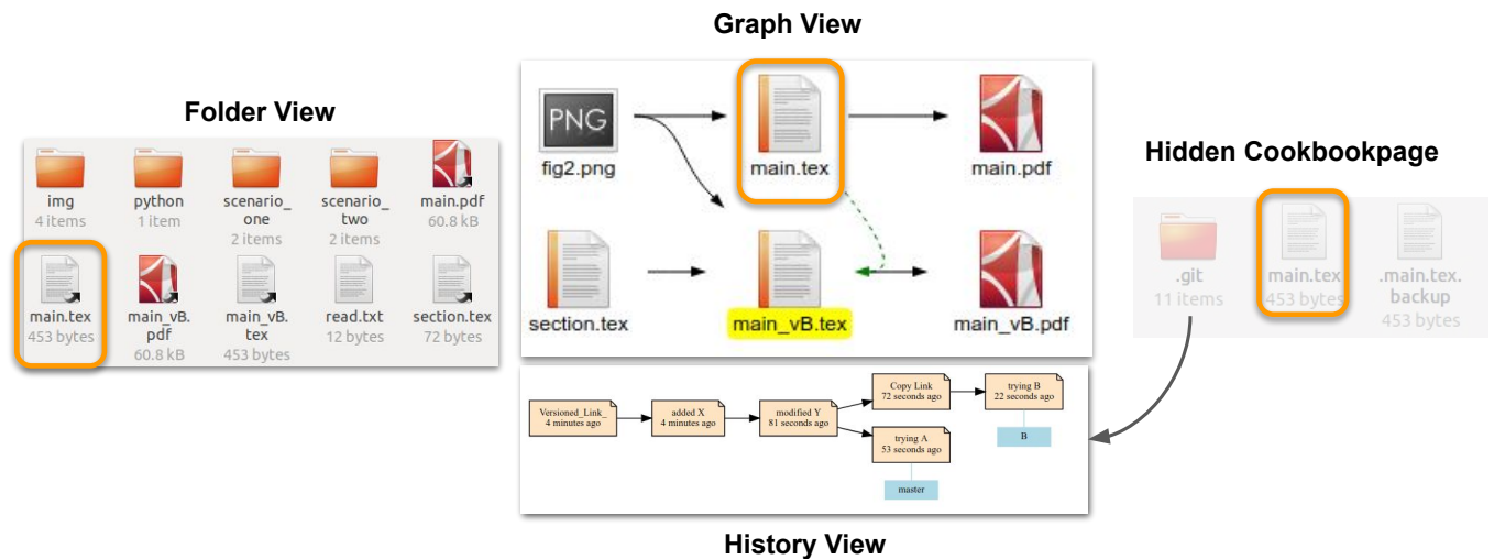
Figure 1. The FileWeaver User Interface. The Folder View (left) is a standard file browsing window. Files with arrows are symbolic links, meaning that they are managed by FileWeaver. The Graph View (center top) was displayed by selecting main.tex in the Folder View, and shows the dependency graph for that file. main_vB.tex is a copy of main.tex (green arrow); both files include fig2.png and section.tex, and they each produce a PDF file. The History View (center bottom) shows the history of versions of main.tex, including the branch that led to main_vB.tex. The Hidden Cookbookpage (right) holds the actual file and its version repository, together with bookkeeping information.
