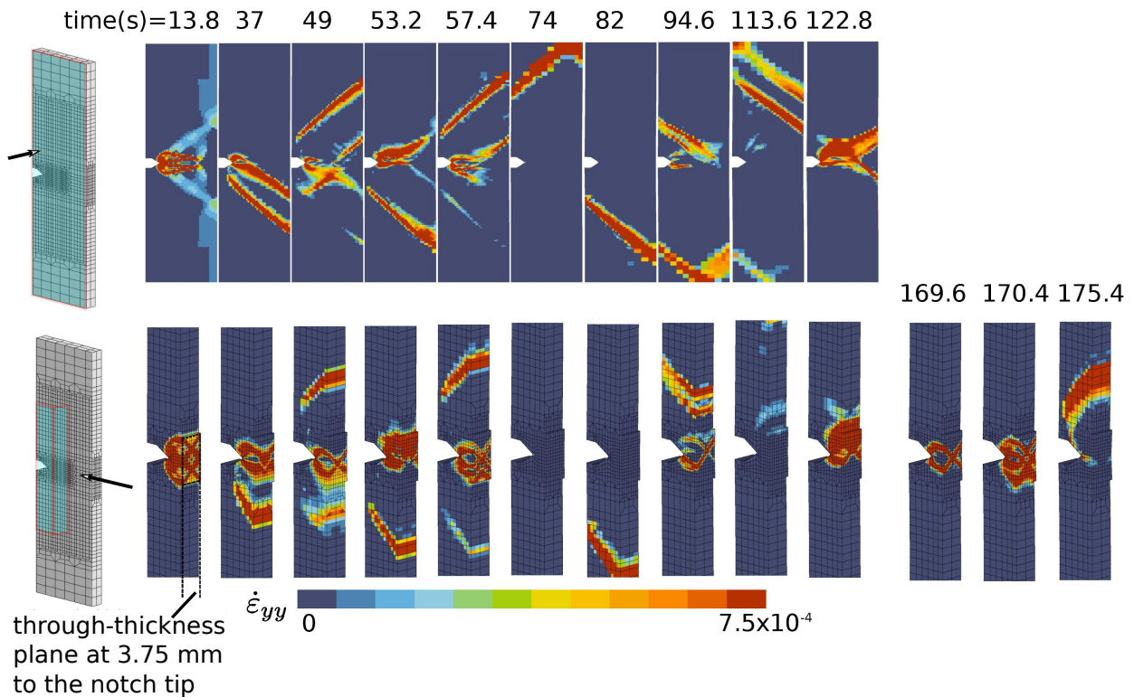
(b) 175 °C; v = 0.01 \text{ mm/s} .
