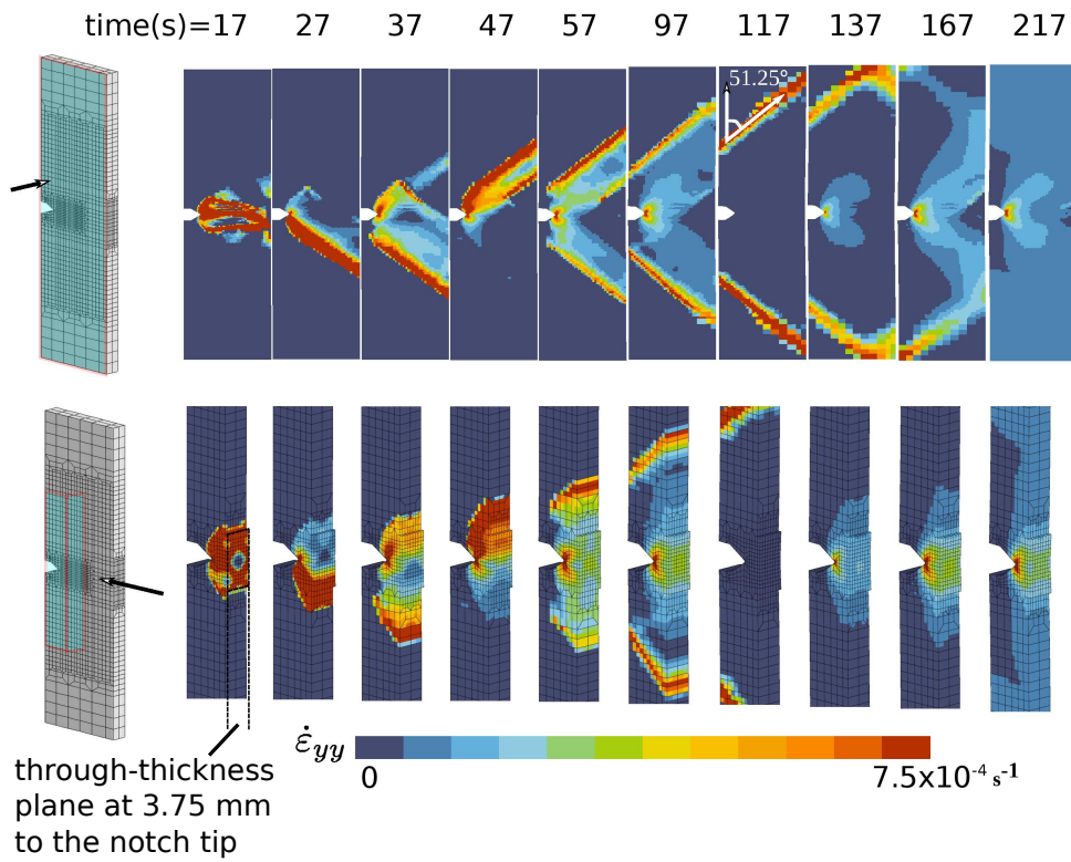
(a) 20 °C; v = 0.01 \text{ mm/s} .
