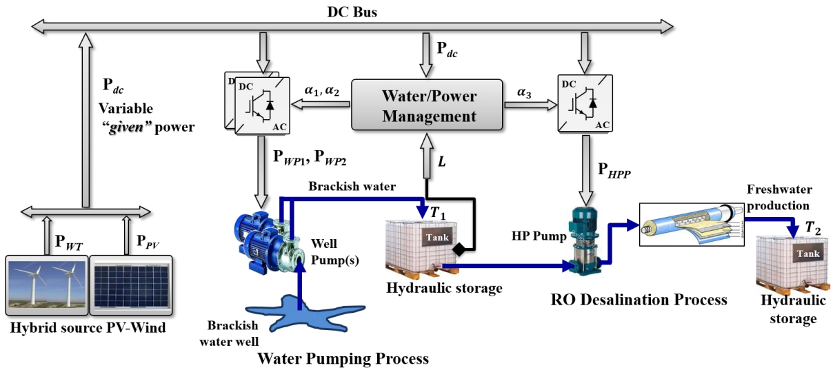
Fig. 1. Synoptic of the autonomous BWRO desalination system
