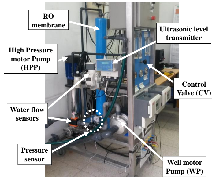
Fig.3. Experimental BWRO desalination test bench
