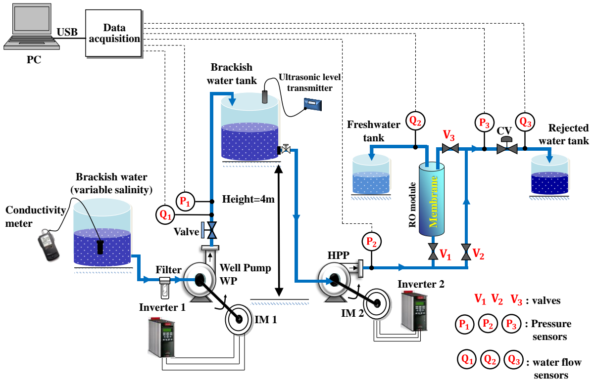
Fig.4. Synoptic scheme of the experimental BWRO desalination test bench
