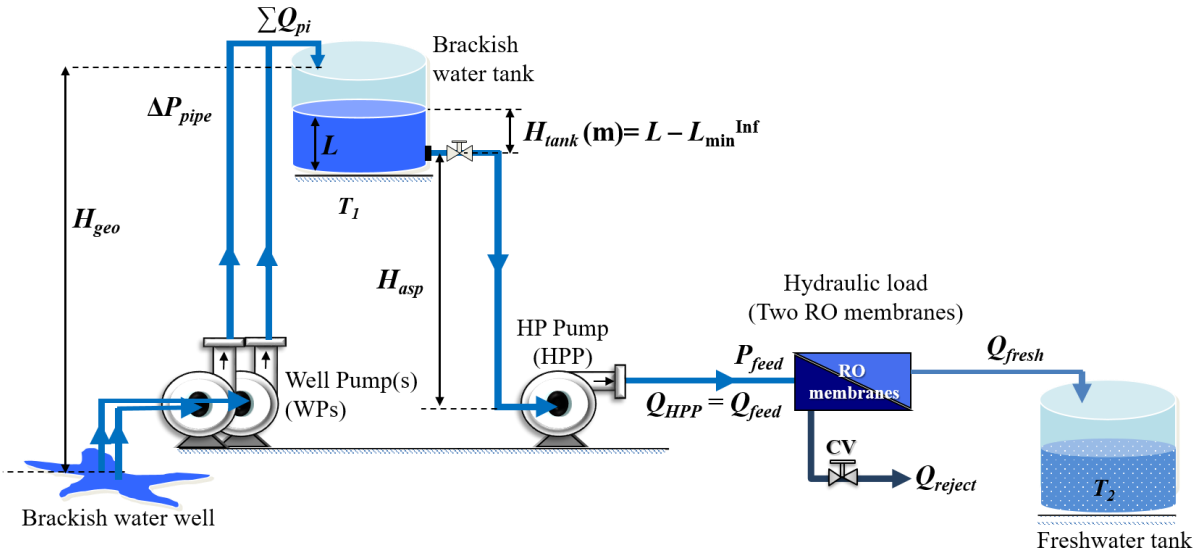
Fig. 2. Hydraulic configuration of the BWRO desalination system
