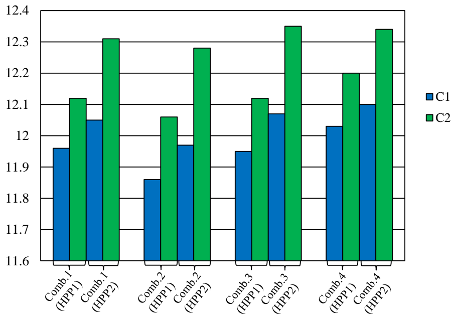
Fig.12. Produced freshwater quantity (in m 3 ) for the different pump-combinations for a daily power profile.
