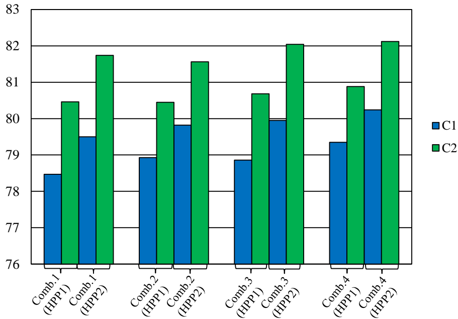
Fig.13. Produced freshwater quantity (in m 3 ) for the different pump-combinations for a weekly power profile.
