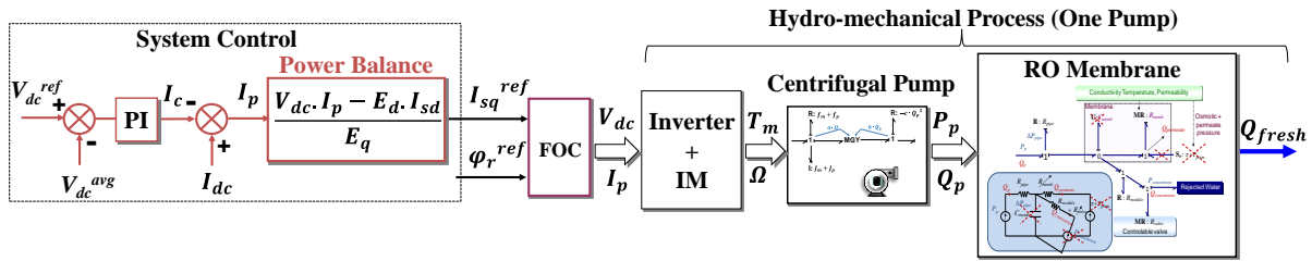
274 Fig.7. Block diagram of the control strategy of a single-pump hydro-mechanical process
