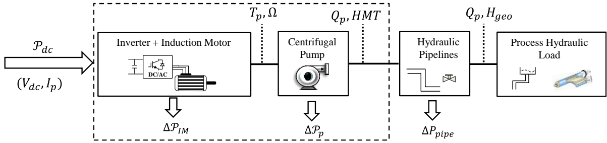
222 223 Fig. 6. Synoptic of the quasi-static modeling of a single-pump hydro-mechanical process: a power flow model
