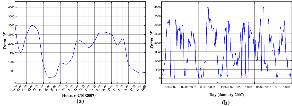
Fig.11. Daily (a) and weekly (b) PV-Wind generated electrical power profiles
