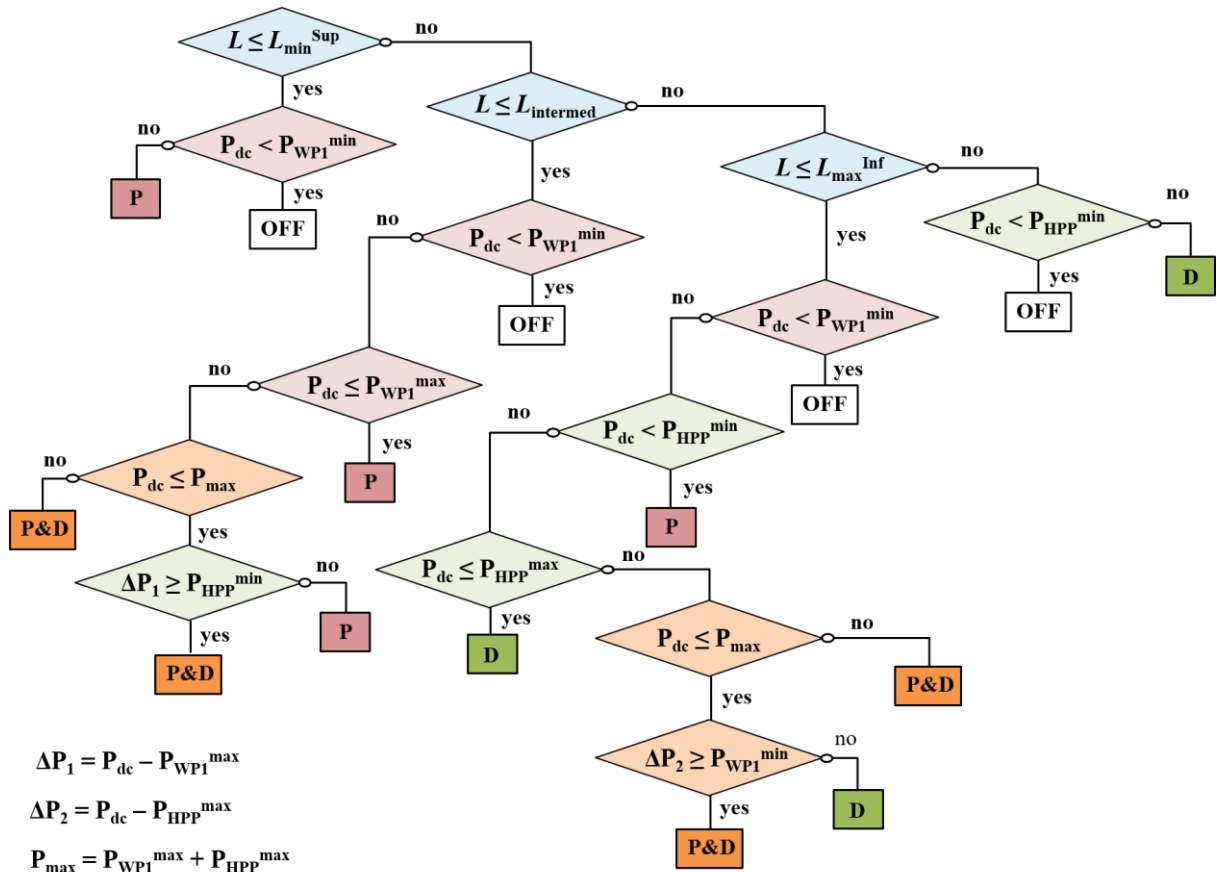
Fig.10. Flowchart of the Deterministic Rule-based energy management strategy for Comb.1
