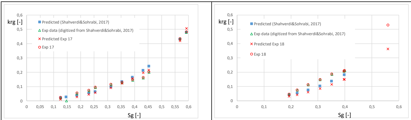
Fig. D3. Comparison of three-phase gas relative permeability as function of gas saturation measured from Oak's DDI Experiment 17 (G2) and that predicted with the mechanistic model. Fig. D6. Comparison of three-phase gas relative permeability as function of gas saturation measured from Oak's DDI Experiment 18 (G3) and that predicted with the mechanistic model.
