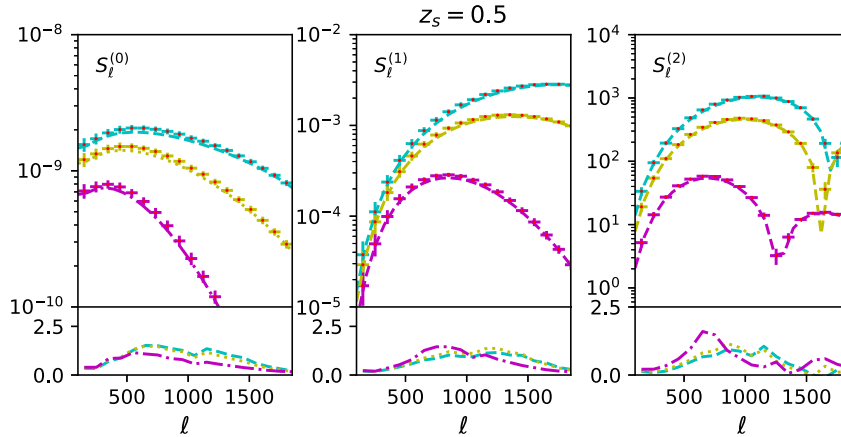
Figure 1. From left to right, different panels depict the skew spectra S_\ell^0 , S_\ell^{(1)} , and S_\ell^{(2)} , respectively, as a function of \ell . The data points with error bars in each panel are the bin-averaged values of the respective skew spectra estimated from simulations. Different curves in each panel correspond to different smoothing angular scales. These generalized skew spectra are defined in equations (15a–15c). In each panel, three different smoothing angular scales \theta_s = 2, 5, and 10 arcmin (from top to bottom) are shown. The source redshift is fixed at z_s = 0.5 . A Gaussian smoothing window was used. See the text for more details. The bottom subpanels for each panel show the deviation \Delta_\ell of simulations S_\ell^{\text{sim}} from theoretical prediction S_\ell^{\text{th}} in units of standard deviation \sigma_\ell computed for individual beams, i.e. \Delta_\ell = (S_\ell^{\text{th}} - S_\ell^{\text{sim}})/\sigma_\ell . No noise or mask was used. For S_\ell^2 , the absolute value |S_\ell^2| is shown in the third panel; the dip feature in this case signifies a zero crossing.
