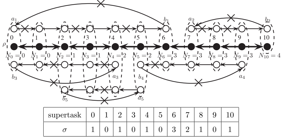
Figure 8: A ZigBee-chain solution: by removing the crossed arcs we obtain the retiming graph \mathcal{R}^\alpha . A corresponding grouped retiming graph \mathcal{G}^\alpha is represented by the filled in black nodes and bold arcs. A core schedule of the supertasks satisfying the precedence constraints of \mathcal{G}^\alpha is shown.
